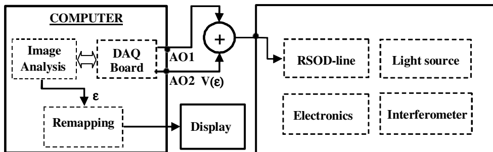
Fig. 2. Schematic of the AR implementation in a standard OCT system.
