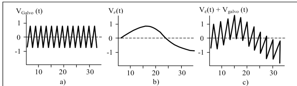
Fig. 4. RSOD Galvanometer driving waveforms. a)- Non AR regime; b) Offset signal; c) AR-regime - summation of the offset with the triangle waveform.
