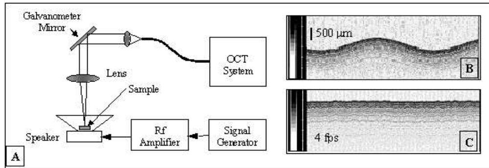
Fig. 10. A. Experimental setup for measurement of the AR performances; B. OCT image without AR; C. OCT image with the AR turned "on". Gray scale bars in B and C represent OCT signal intensity.
