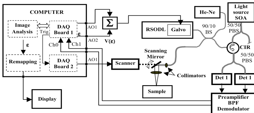
Fig. 6. Schematic of the MGH AR TD-OCT System. SOA –Semiconductor Optical Amplifier, \Sigma -summator, PBS-Polarization Beam splitter; BS-beam splitter, BPF-Band Pass Filter.
