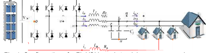
Fig. 1. Configuration of a FL-VSI based standalone power supply.
