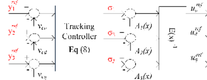
Fig. 3. Feedback linearization control block diagram.
