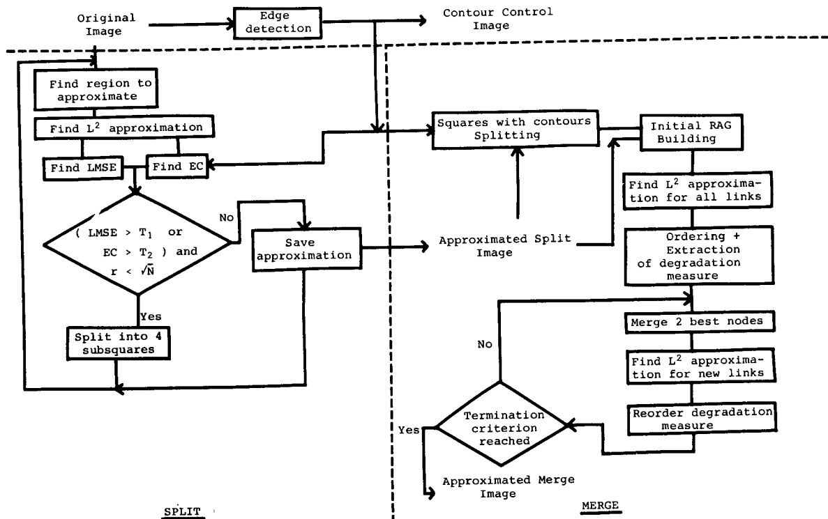
Figure 1 : Segmentation process.
