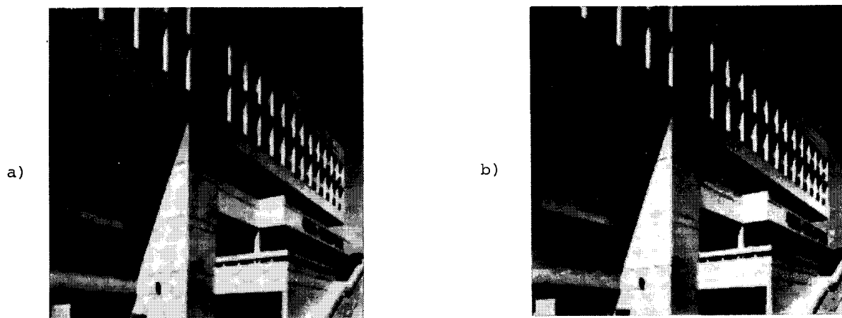
Fig. 6 : Building picture with an approximation by planes 6a) split approximated image (6688 squares). 6b) LMSE merge approximated image (999 regions).
