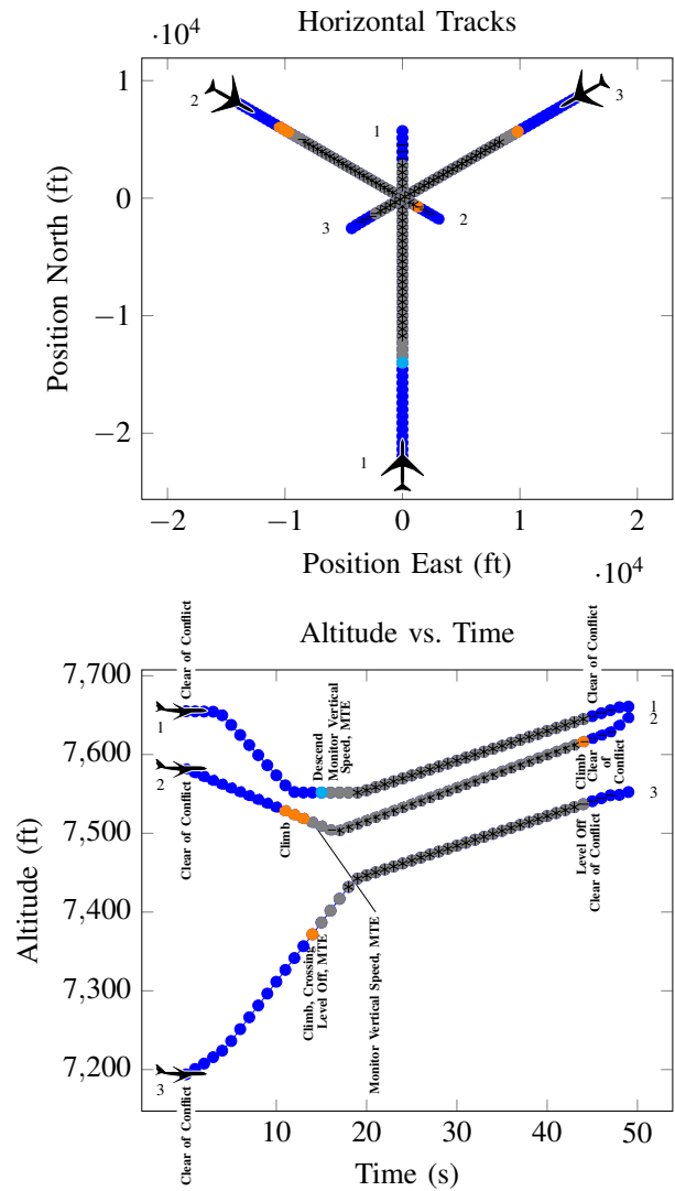
Figure 7. NMAC Related to Pairwise Coordination
