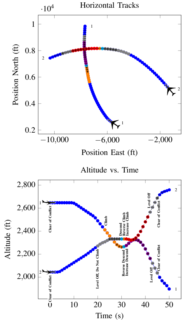
Figure 5. NMAC Related to Crossing Time
