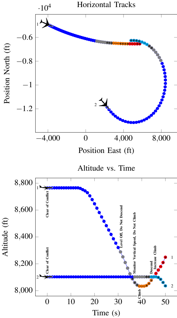
Figure 6. NMAC Related to High Turn Rate
