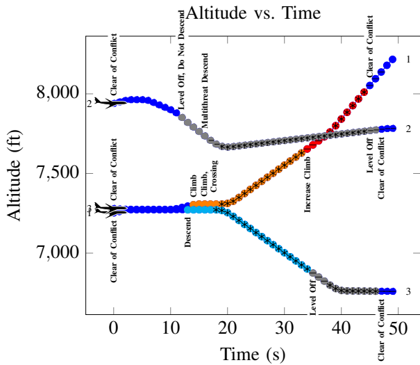
Figure 8. NMAC Related to Reduced Airspace
