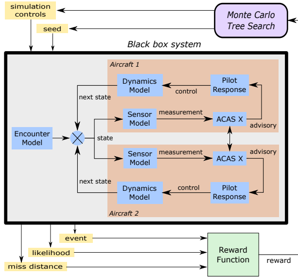
Figure 4. System Diagram for Pairwise Encounters
