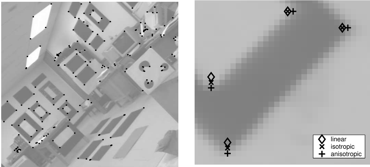
Figure 16: LEFT: Corners detected in the ‘lab’ test image using the nonlinear structure tensor with anisotropic diffusion. RIGHT: Comparison of the corners detected by the classic linear structure tensor and the nonlinear structure tensor with an underlying isotropic and anisotropic diffusion process, respectively.
