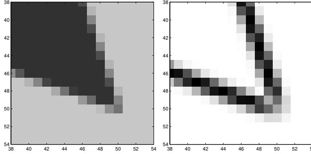
Figure 14: LEFT: Detail of a test image with ideal corner position (50, 50). RIGHT: Larger eigenvalue of the unsmoothed structure tensor J_0 .
