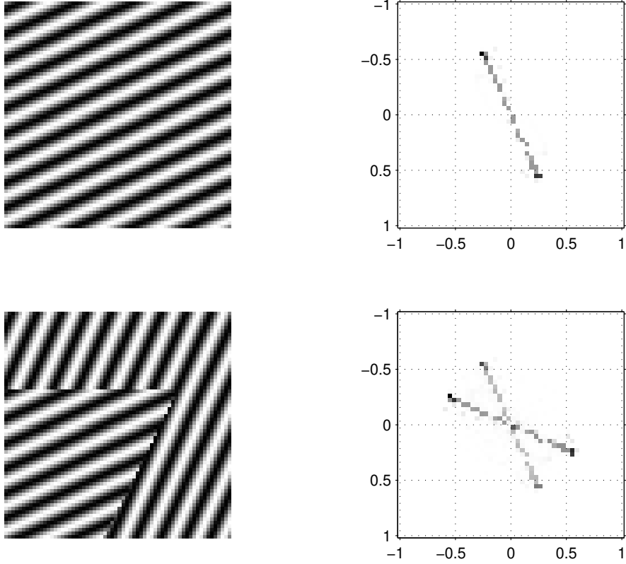
Figure 1: Histograms of gradient vector space. In (a) an image ( 64 \times 64 ) is shown with in (b) the histogram of all gradient vectors (where darker shades indicate that those gradient vectors occur more often in the image). In (c) a composition of two differently oriented patterns is shown with the corresponding histogram in (d).
