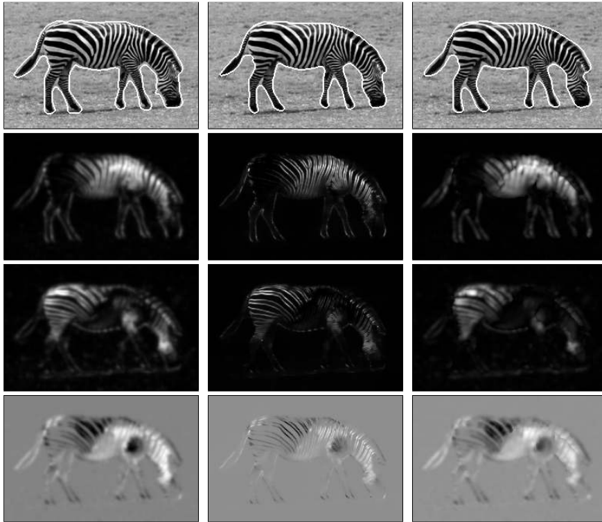
Figure 12: LEFT COLUMN: Segmentation with the classic structure tensor ( \rho = 2 ). CENTER COLUMN: Segmentation with the nonlinear structure tensor ( t = 25 ). RIGHT COLUMN: Segmentation with the robust structure tensor ( \rho = 3, m = 0.05 ). FROM TOP TO BOTTOM. (a) Segmented image ( 250 \times 167 ). (b) Tensor component J_{11} based on I_x^2 . (c) J_{22} based on I_y^2 . (d) J_{12} based on I_x I_y .
