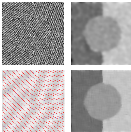
Figure 11: Comparison between least squares and robust orientation estimation. See also colour plates.
