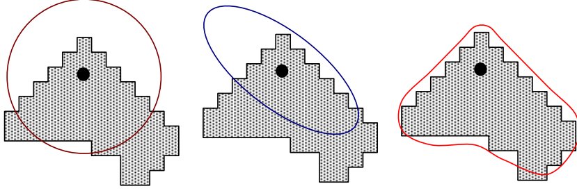
Figure 4: LEFT: Neighborhood of a non-adaptive isotropic Gaussian. CENTER: Neighborhood of a data-adaptive anisotropic Gaussian. RIGHT: Neighborhood obtained with an iterative diffusion process.
