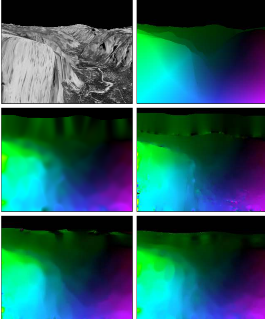
Figure 7: Yosemite sequence without clouds ( 316 \times 252 \times 15 ). FROM LEFT TO RIGHT, TOP TO BOTTOM: (a) Frame 8. (b) Ground truth. (c) Classic structure tensor. (d) Nonlinear structure tensor. (e) Robust structure tensor. (f) Coherence based smoothing. See colour plates.
