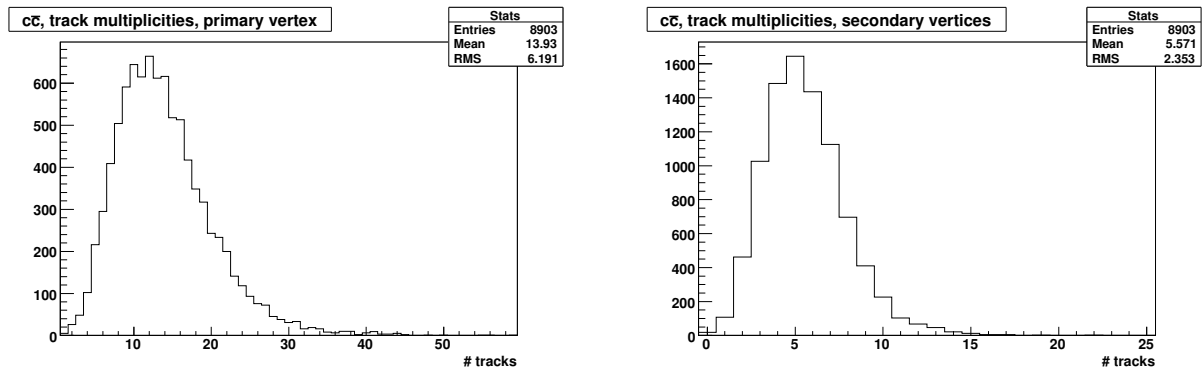
Figure 4: Reconstructed track multiplicities in the c\bar{c} sample — primary vertex (left) and secondary vertices (right). Note that the track multiplicities of the secondary vertices are the multiplicities of the sum of all secondary vertices per event.
