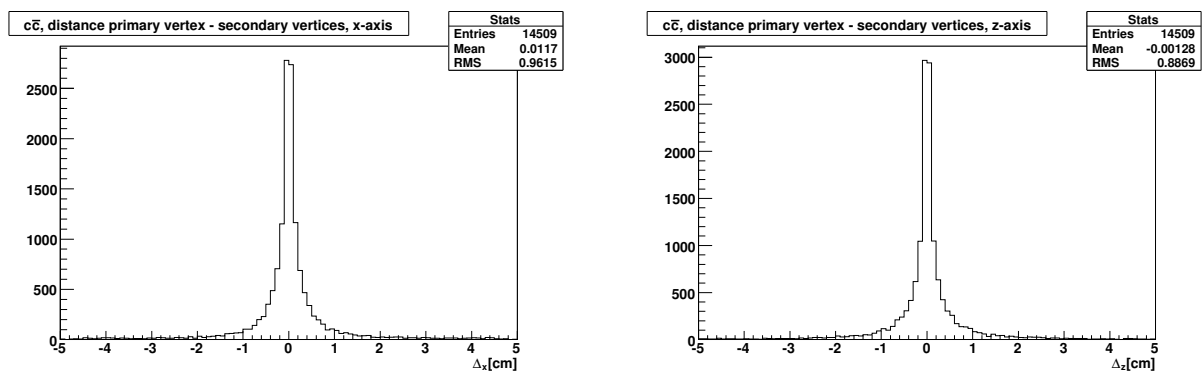
Figure 5: Distances between simulated collision (primary) vertices and decay (secondary) vertices in the c\bar{c} sample.
