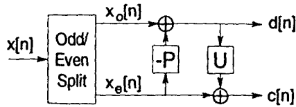
Figure 1: Lifting stage: Split, Predict, Update.
