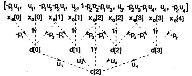
Figure 3: Update filtering. An N = 2 point linear predict followed by an \tilde{N} = 4 point linear update yields the update vector \mathbf{h} shown across the top.
