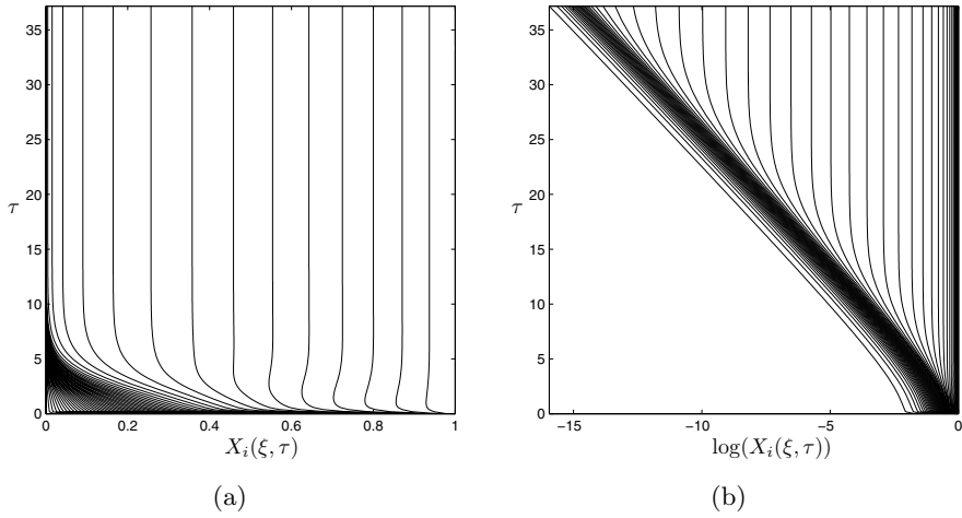
Figure 5.4. Example 2 . Blow-up mesh. (a) Grid in the natural coordinates. (b) Plotting \tau = |\log(T - t)| as a function of \log(X_i) at equally spaced values of \xi , showing the contraction rate and approximately self-similar behaviour close to the origin.
