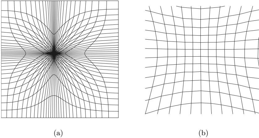
Figure 5.2. Example 1. Final grid for the blow-up example. (a) Entire grid. (b) Detail near the blow-up point. Note that the grid is quite regular in the vicinity of the singularity, with no evidence of any skewness or tangling.
