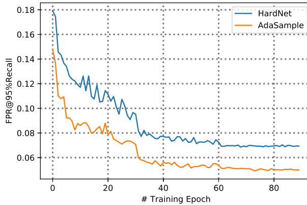
Figure 4: Training trend of AdaSample and HardNet (Mishchuk et al., 2017) on HPatches (Balntas et al., 2017) dataset.
