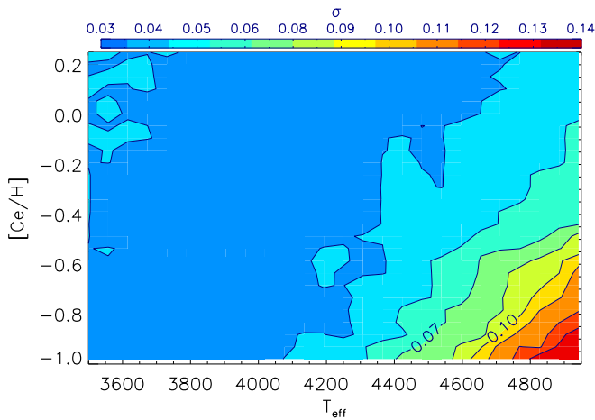
Figure 9. Contour plot of the uncertainties (in dex) of [Ce/H] as a function of T_{\text{eff}} and \log g (with each T_{\text{eff}} paired with a corresponding \log g along the red giant branch; same as Figure 8). The calculations are done for the \lambda 16376 \text{ \AA} Ce II line, the same Ce II line as used in Figure 8, and the APOGEE spectra with S/N = 100 .
