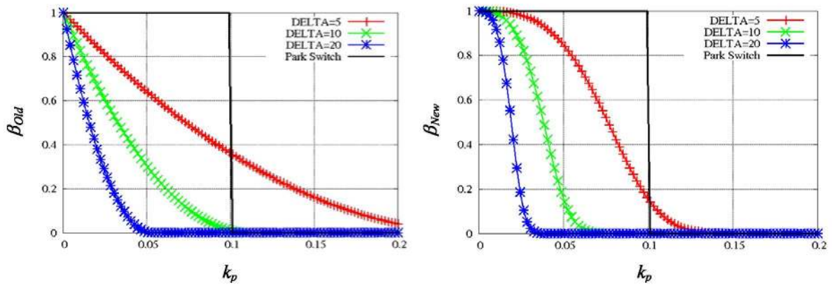
Figure 3. Switching functions for the HLLC+ and HLLC+ algorithms.
