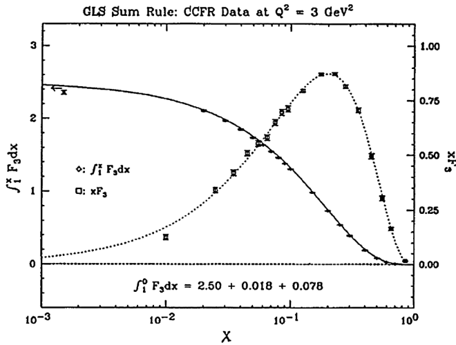
FIG. 2. Experimental results for Gross–Llewellyn Smith sum rule, Eq. (10), from the CCFR group, Ref. [4]. All data have been interpolated or extrapolated to Q^2 = 3 \text{ GeV}^2 . Squares: x\bar{F}_3(x) , sum of neutrinos plus antineutrinos, at Q^2 = 3 \text{ GeV}^2 . Dashed curve: analytic fit to x\bar{F}_3 . Diamonds: approximation to the integral S_{\text{GLS}}(x) of Eq. (11). Solid line: fit to the integral S_{\text{GLS}}(x) .
