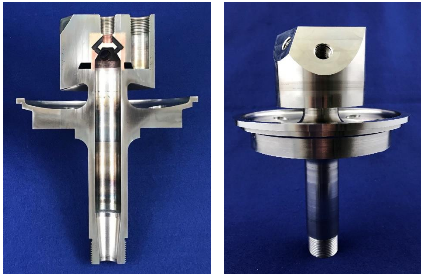
Figure 36. Bi-metallic prototype of the RS-25 ASI, built using hybrid manufacturing. (Left) A cross section of the first full build of the ASI with no fuel orifices. (Right) the final hot-fire version that included fuel orifices.
