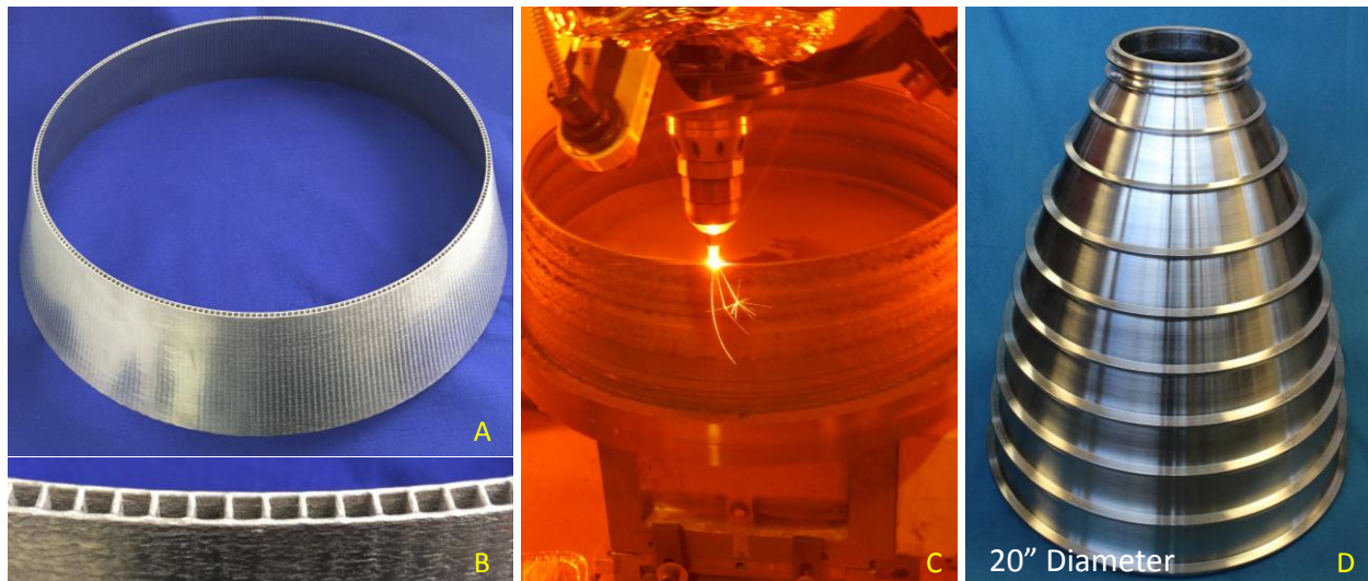
Figure 5. Nozzle feasibility demonstrator components fabricated with DED blown powder deposition – A. Channel wall nozzle MTD with integral channels, B. Integral Channels Fabricated, C. In-process DED fabrication of subscale nozzle jacket, D. Final-machined DED blown powder nozzle jacket.
