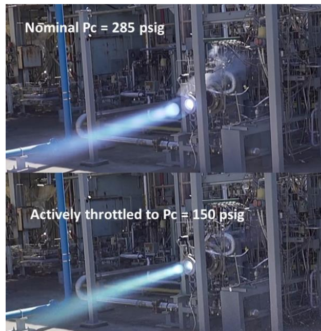
Figure 16. Active Throttling Successfully Demonstrated on META4 #2.
