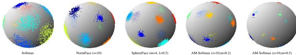
Figure 5: Feature distribution visualization of several loss functions. Each point on the sphere represent one normalized feature. Different colors denote different classes. For SphereFace Liu et al. (2017a), we have already tried to use the best hyper-parameters we could find.
