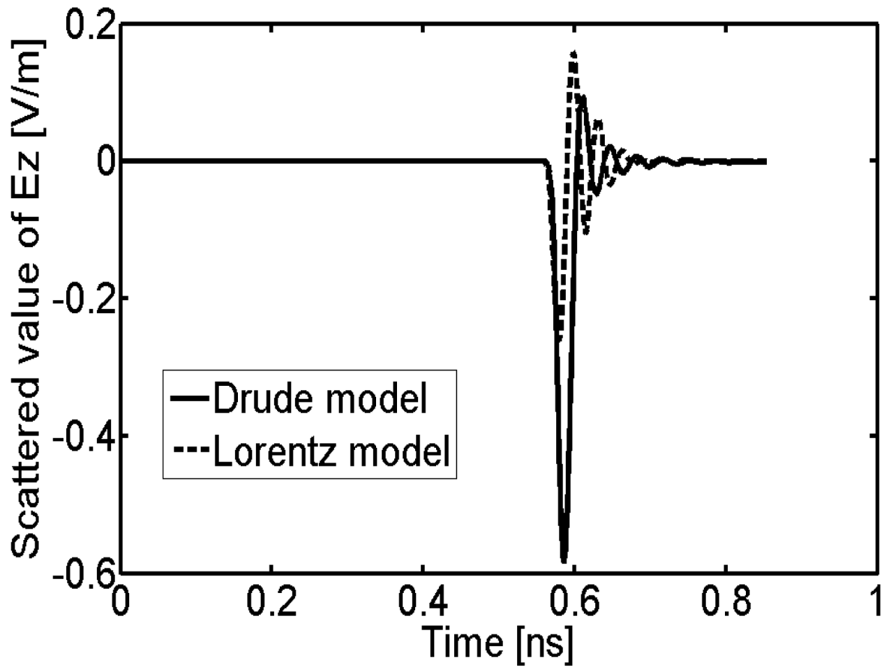
Fig. 1. FDTD-calculated time-waveforms of the scattered (reflected) electric field for both the Drude and Lorentz half-space examples. The maximum Gaussian incident value is set to 1 V/m.
