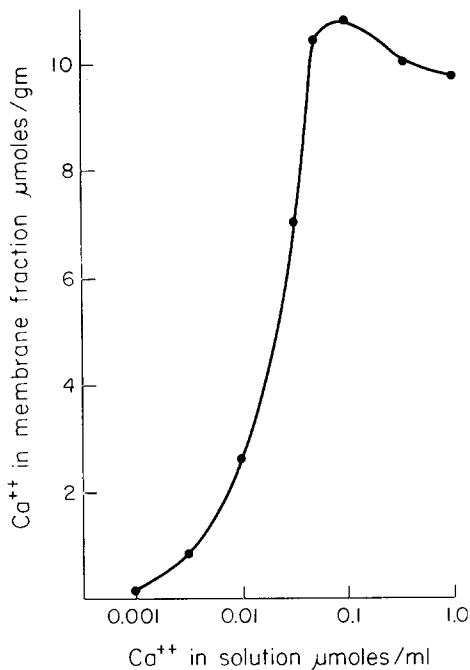
FIGURE 4 Calcium ion binding of membrane fraction as a function of calcium concentration in solution. Each ml of solution contained 2.0 mg of membrane fraction. See Methods for further details.
