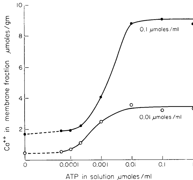
FIGURE 5 Calcium ion binding of membrane fraction as a function of ATP concentration in solution. Each ml of solution contained 2 μmoles of PEP, 140 units of pyruvate kinase, 1.0 mg of membrane fraction and either 0.1 or 0.01 μmoles per ml of calcium ion. See Methods for further details.
