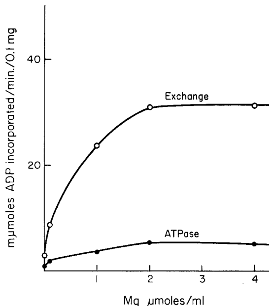
FIGURE 10 Effect of varying concentrations of magnesium ion on the ATP-ADP exchange reaction and ATPase of the particulate fraction. 0.1 mg per ml of membrane fraction was used in each case. See Methods for details.
