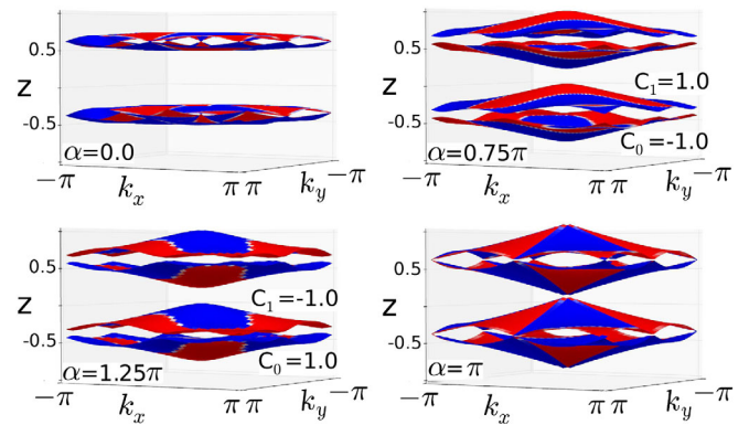
FIG. 1 (color online). The two WCC sheets of the half filled FKM model, and one set of periodic images, at four stages \alpha = (0, 3\pi/4, \pi, 5\pi/4) along the parametric cycle (clockwise from upper left). Blue and red colors show positive and negative values of Berry curvature \Omega_z on the sheets, respectively. The Chern numbers associated with the individual WCC sheets are shown for those cases where sheets do not touch.
