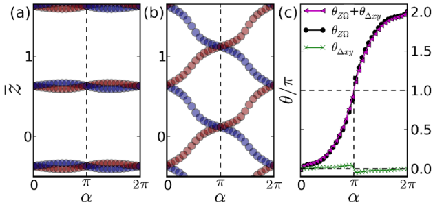
FIG. 2 (color online). WCCs at (a) M and (b) \Gamma of the 2D BZ for the FKM model as a function of the adiabatic loop parameter \alpha . Blue and red colors indicate positive and negative values of Berry curvature, respectively. (c) CSA coupling \theta(\alpha) and its contributions \theta_{z\Omega} and \theta_{\Delta xy} for the same adiabatic loop.
