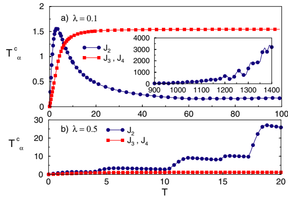
FIG. 1 (color online). T_\alpha^c as a function of T for the Jordan blocks J_2 , J_3 , and J_4 . The inset of (a) shows that J_2 has non-negligible couplings for T \sim 10^3 (in units such that \omega = 1 ).
