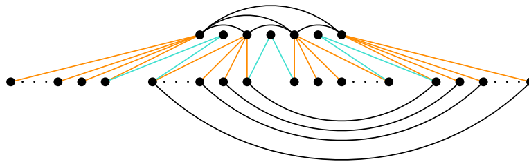
Figure 13: Illustration of the construction showing that we cannot keep more than a quarter of the external adjacencies. Black edges indicate internal adjacencies; orange and blue edges are external adjacencies. Blue edges are incident to an isolated vertex in the top graph.
