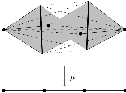
FIGURE 3. \mathbb{P}^1 \times \mathbb{Q} with \mathbb{C}^* action
