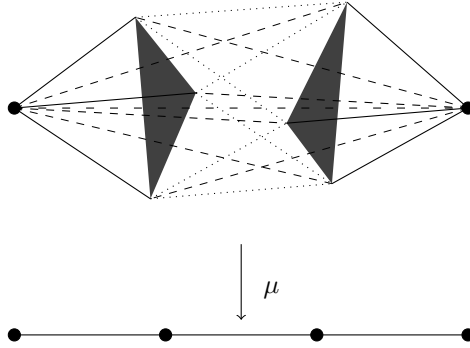
FIGURE 4. The \mathrm{Sp}_6 homogeneous variety
