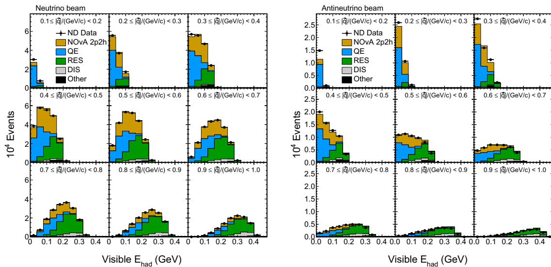
Fig. 8 Comparison of fully adjusted simulation to ND data in reconstructed visible hadronic energy for neutrinos (left) and antineutrinos (right). The panels show 0.1 GeV/c wide bins of reconstructed momentum transfer from 0.1–0.2 GeV/c (upper left) to 0.9–1.0 GeV/c (lower right)
