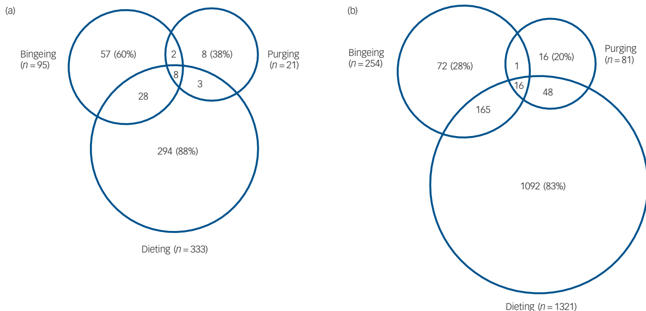
Fig. 1 Co-occurrence of eating disorder behaviours across genders: (a) boys ( n = 2688 ); (b) girls ( n = 3374 ).
