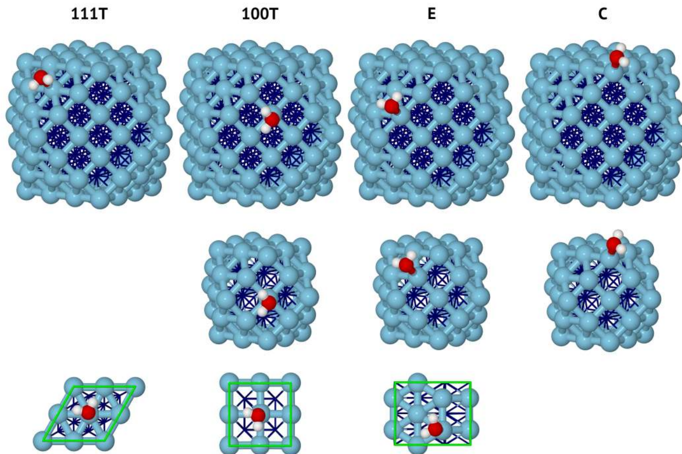
36 37 38 39 40 41 42 43 44 45 46 47 48 49 Figure 2: Adsorption modes of molecular water on each studied surface site (bulk metal atoms in dark blue, surface metal atoms in light blue, oxygen in red, hydrogen in white, unit cells of the extended surfaces in green). See Figure 1 for the notation of the surface sites.
