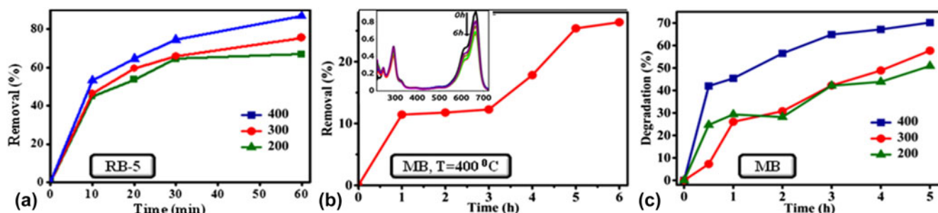
FIG. 5. (a) Effect of annealing temperature of NiO NPs on RB-5 removal efficiency, (b) NiO NPs were tested for the MB removal efficiency (annealing temperature of sample is 400 °C) and the inset of this figure shows UV-visible absorption spectra for the adsorption of MB over NiO NPs in the absence of visible light, and (c) comparative analysis of MB degradation efficiency over NiO NPs in the presence of visible light.
