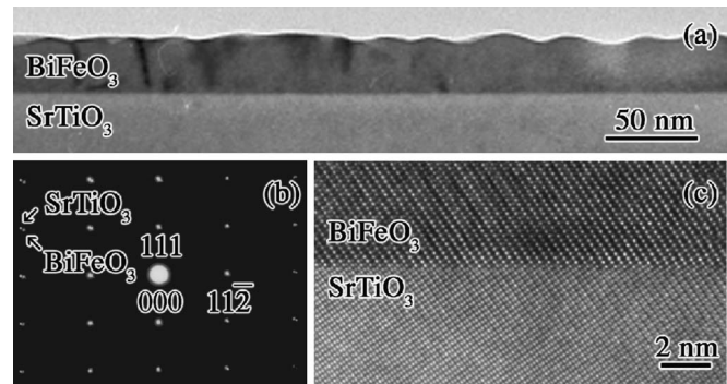
FIG. 2. (a) Bright-field TEM image of the same film whose XRD is shown in Fig. 1. (b) Selected-area electron diffraction from region covering the film and the substrate. Reflections from the SrTiO 3 substrate are indexed. (c) HRTEM image of the film/substrate interface.
