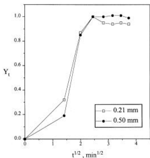
Figure 5. Time-dependence of the fraction of adsorption at different particle sizes of chitosan.
