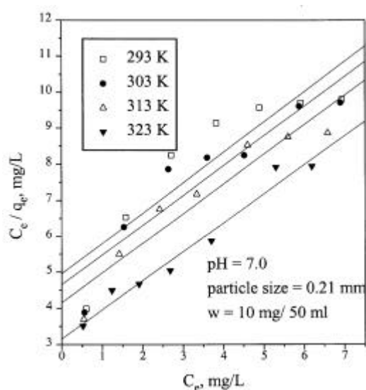
Figure 10. Langmuir isotherm.
