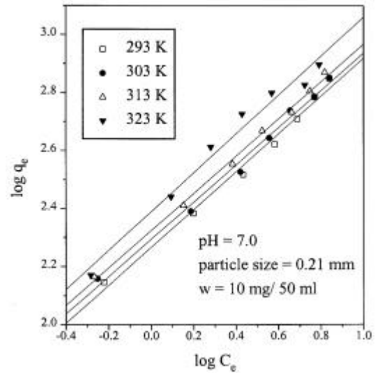
Figure 9. Freundlich isotherm.
