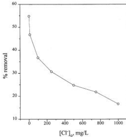
Figure 4. Effect of chloride ion concentration.
