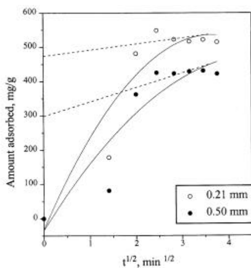
Figure 7. Intraparticle diffusion plot for the adsorption of zinc on chitosan at different particle sizes.
