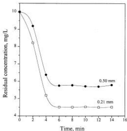
Figure 1. Effect of particle size.
