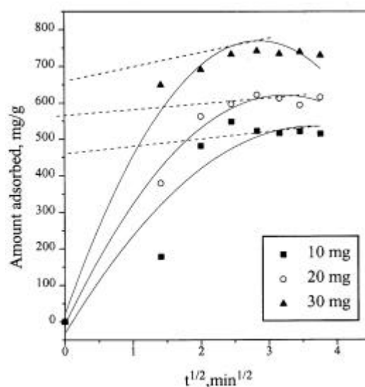
Figure 8. Intraparticle diffusion plot for the adsorption of zinc on chitosan at different dosages.
