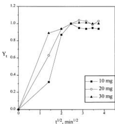
Figure 6. Time-dependence of the fraction of adsorption at different amounts of chitosan.
