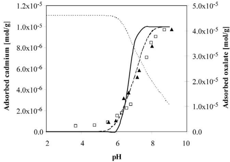
Figure 3. pH adsorption-edge of Cd on goethite in the presence of oxalate (▲). A reference experiment performed in 0.01 M KNO 3 (□), could be described by the SCM and the DLM (---). The calculated oxalate adsorption-edge in the presence of Cd is represented (-----). Cd adsorption in the presence of oxalate was calculated with approach 1 (—).
