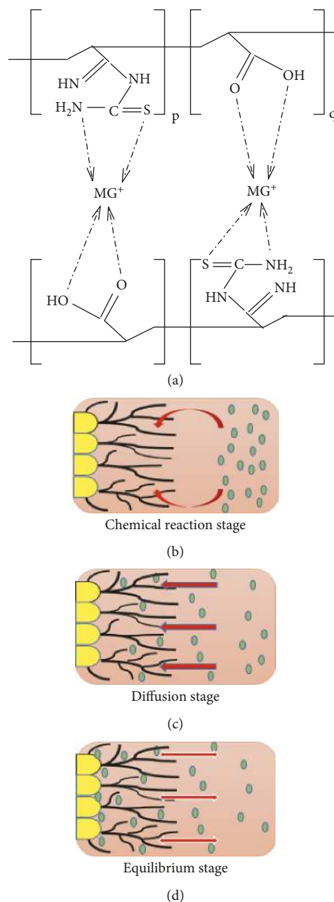
FIGURE 10: Proposed adsorption mechanism (a) and kinetic process (b-d).
