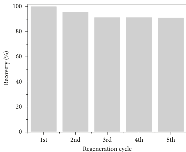
FIGURE 11: Recyclability of TU-poly(AN-co-AA) for adsorption of MG.
