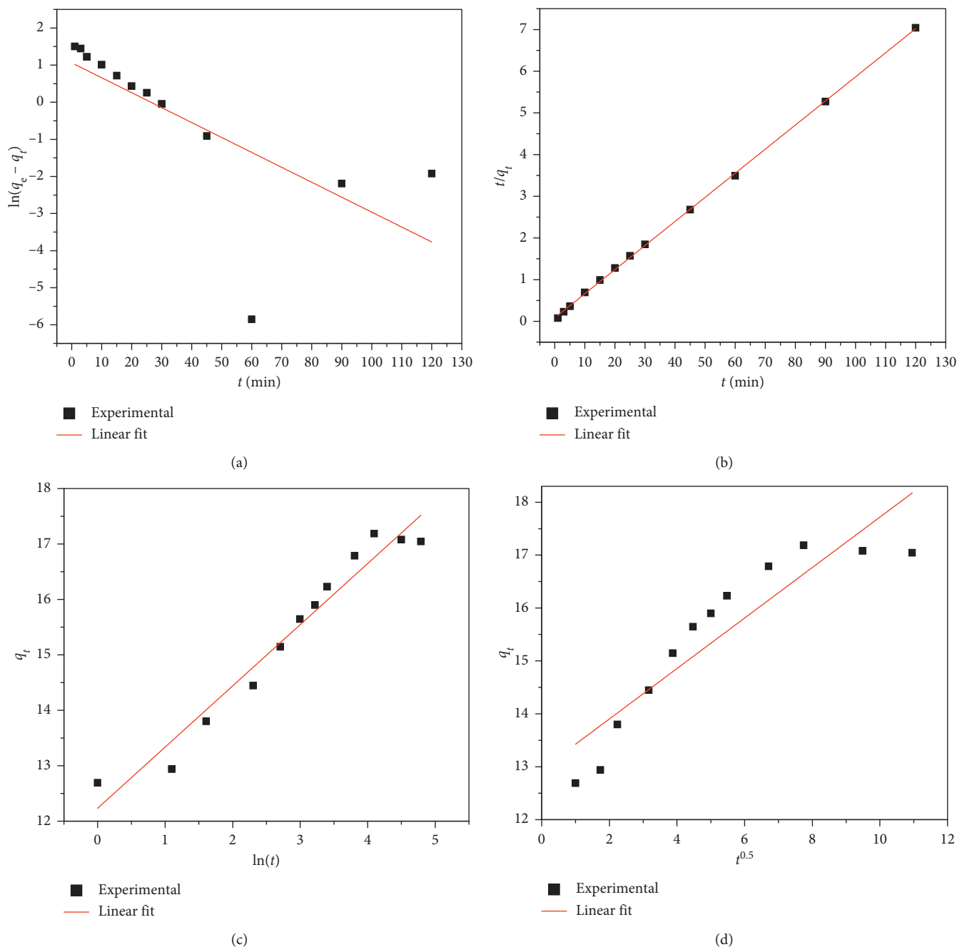
FIGURE 8: Plot of pseudo-first-order (a), pseudo-second-order (b), Elovich kinetic (c), and intraparticle diffusion (d) models.
