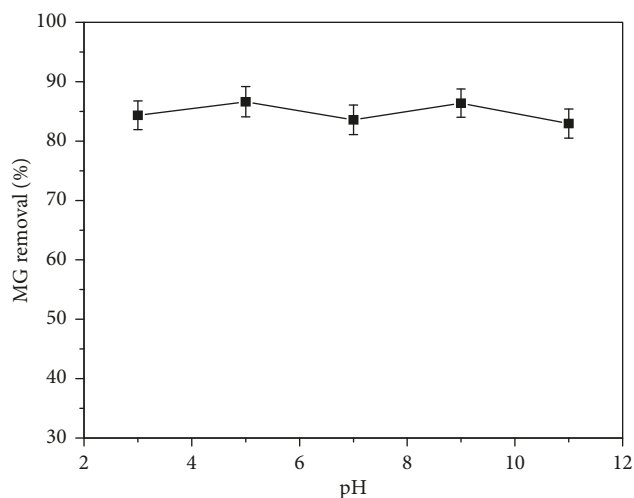
FIGURE 6: Effect of initial pH on MG adsorption onto TU-poly(AN-co-AA) (initial concentration: 50 mg/L; adsorbent dosage: 0.5 g; temperature: 298 K; agitation speed: 100 rpm).
