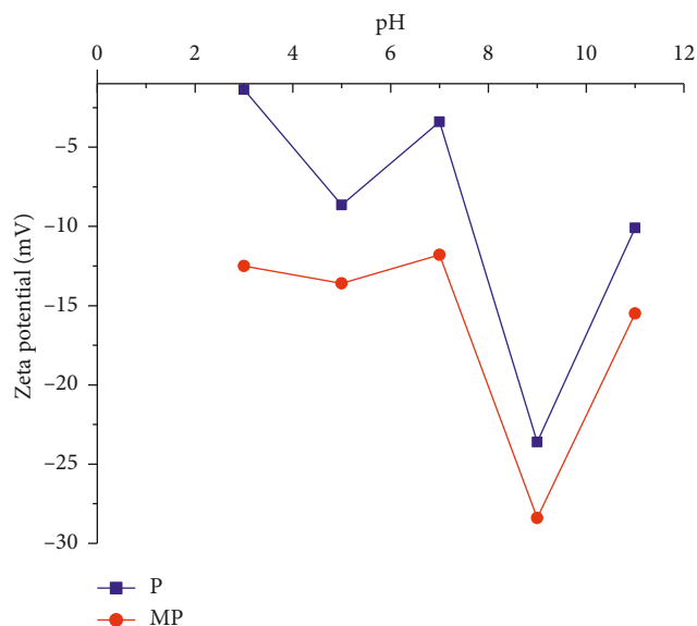
FIGURE 3: Zeta potentials of poly(AN-co-AA) (P) and TU-poly(AN-co-AA) (MP) under different pH values.
