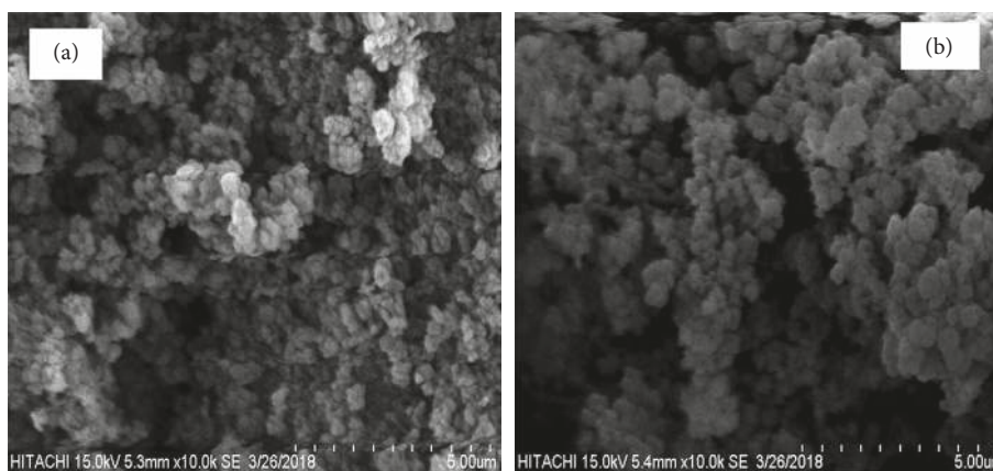
FIGURE 2: SEM micrographs of poly(AN-co-AA) (a) and TU-poly(AN-co-AA) (b).
