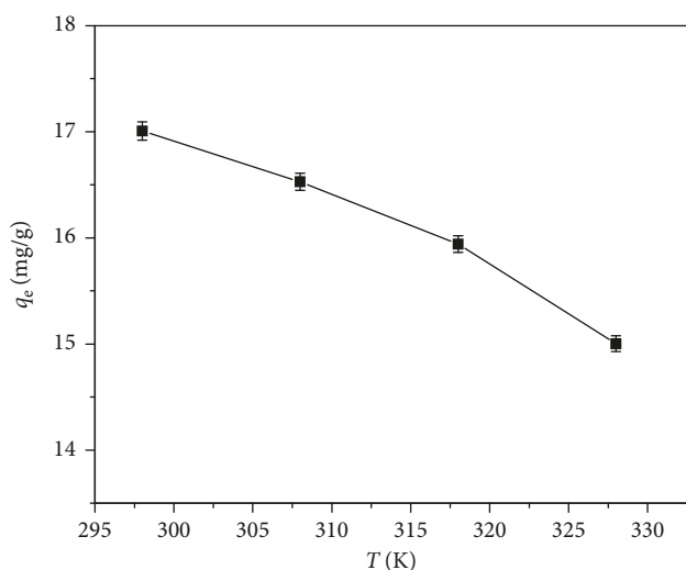
FIGURE 7: Effect of initial temperature on MG adsorption onto TU-poly(AN-co-AA) (initial concentration: 100 mg/L; adsorbent dosage: 0.5 g; agitation speed: 100 rpm).
