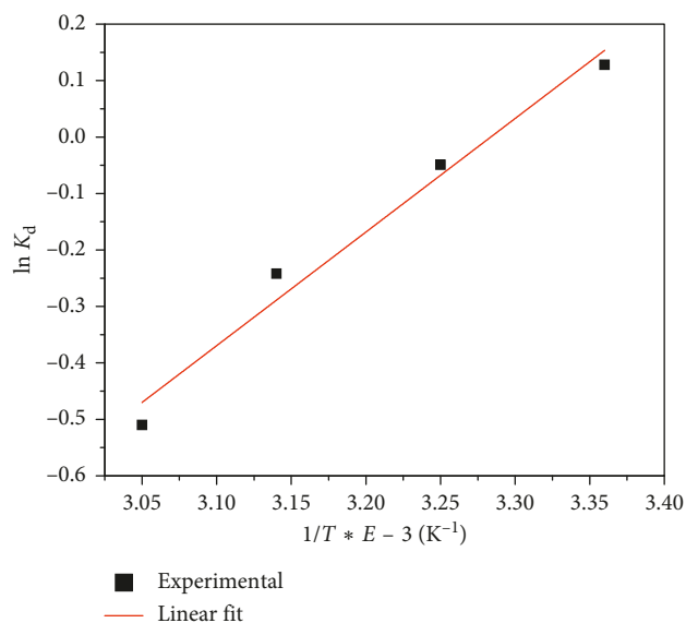
FIGURE 9: Van't Hoff plot for MG adsorption onto TU-poly(AN-co-AA) (MG concentration: 100 mg/L; dosage: 0.5 g; contact time: 60 min; agitation speed: 100 rpm).
