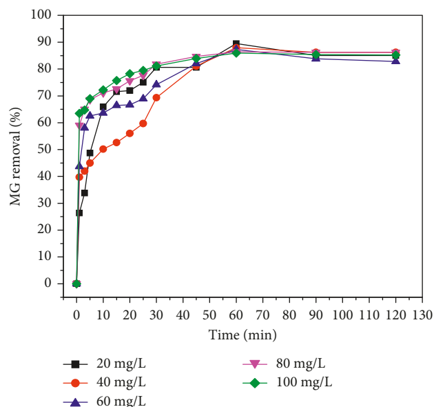
FIGURE 5: Effect of contact time on MG adsorption on TU-poly(AN-co-AA) (adsorbent dosage: 0.5 g; temperature: 298 K; agitation speed: 100 rpm).
