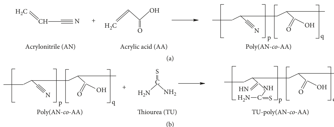
SCHEME 1: Polymerization of poly(AN-co-AA) (a) and modification of poly(AN-co-AA) with thiourea (b).
