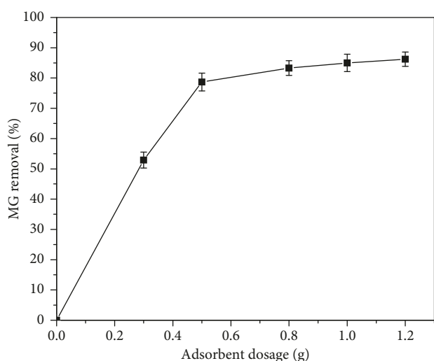
FIGURE 4: Effect of adsorbent dosage on the adsorption of MG onto TU-poly(AN-co-AA) (concentration: 50 mg/L; temperature: 298 K; contact time: 60 min; agitation speed: 100 rpm).
