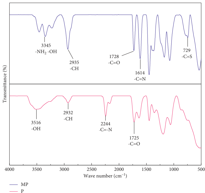
FIGURE 1: FTIR spectra of poly(AN-co-AA) (P) and TU-poly(AN-co-AA) (MP) polymers.
