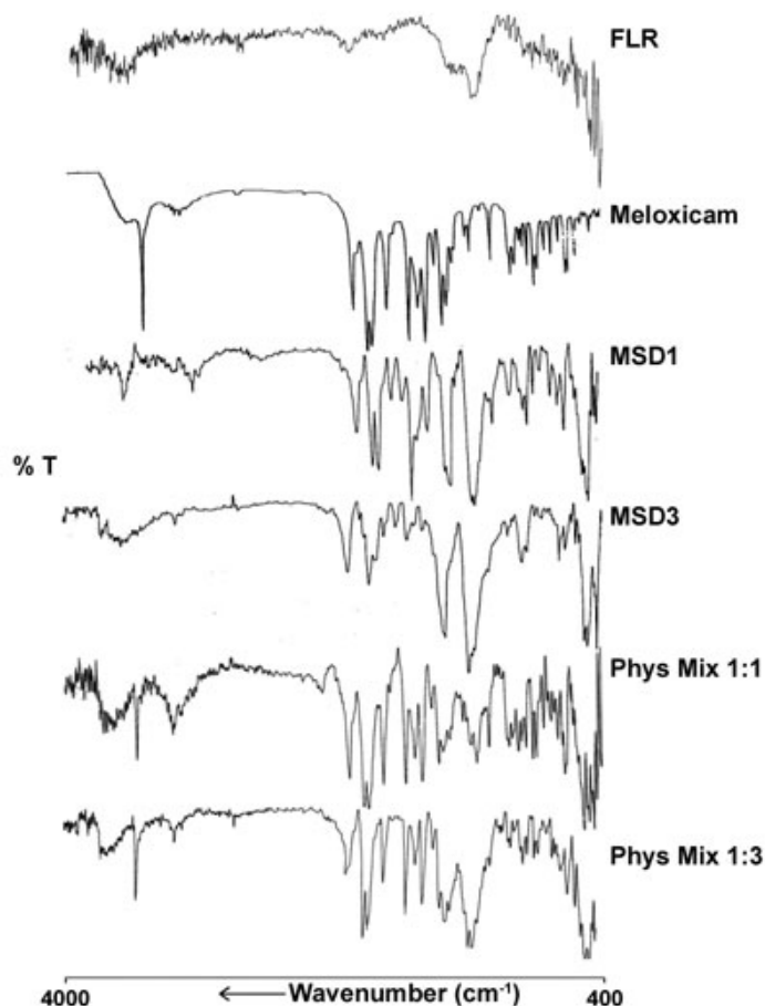
Figure 4. IR of FLR, meloxicam, MSD1, MSD3, and physical mixtures (1:1 and 1:3).
