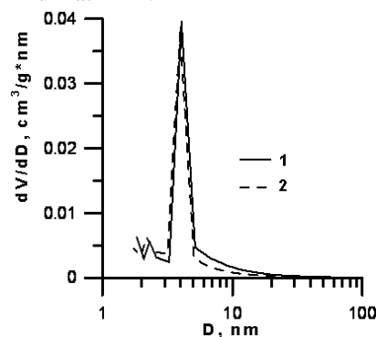
Fig. 5. Pore size distribution curves for the initial bentonite (curve 1) and the composite bentonite-PANI (curve 2)
