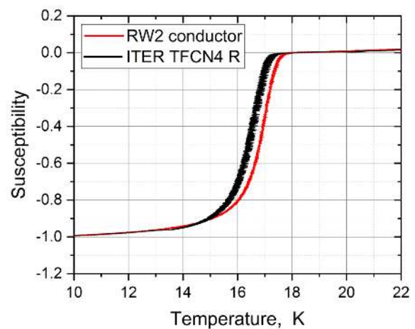
Fig. 8 Susceptibility measured in the DEMO TF RW2 prototype conductor and for the ITER TF SULTAN sample.
