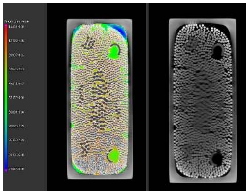
Fig. 6 X-ray computer tomography image of the TF WP#2 conductor prototype with slightly reduced jacket thickness. Left plot
