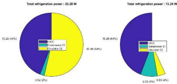
Fig. 5 Cryogenic load for one pancake of the TF WP#3 design before and after the optimization. In the reference scenario (left plot), the helium inlet temperature is 4.45 K and pressure head 1 bar, while in the optimized case (right plot) the inlet temperature is 4.0 K and pressure head 0.2 bar.
