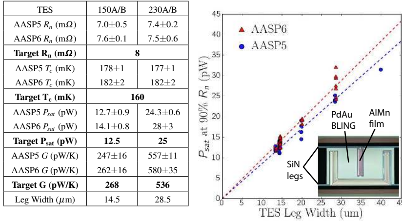
Fig. 2: Left : Measured average and RMS AdvACT detector parameters for many HF single pixels fabricated on two 75 mm test wafers, AASP5 and AASP6, as compared with targeted values. R_n is the AlMn film normal resistance, T_c the transition temperature, P_{sat} the electrical bias power at 90% R_n , and G the thermal conductance to the bath at T_c . Right : P_{sat} versus SiN leg width for typical HF 230/150 and MF 90 GHz devices. Right inset : A microscope image of an AdvACT AlMn TES [34]. (Color figure online.)
