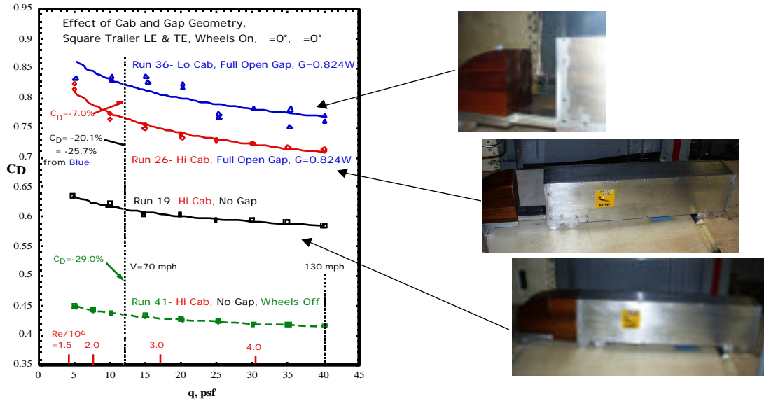
Figure 8 - Phase I Test Results for Unblown Configurations, Showing Effects of Cab Height, Cab/Trailer Gap, Reynolds Number and Wheels
