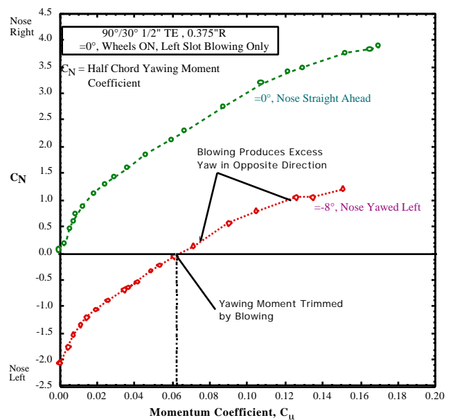
Figure 21 - Directional Control Capability Provided by Blown HV Configuration
