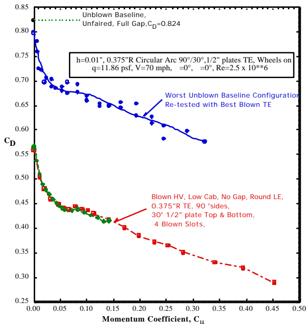
Figure 16 - Additional Drag Reductions and Comparative Configurations
