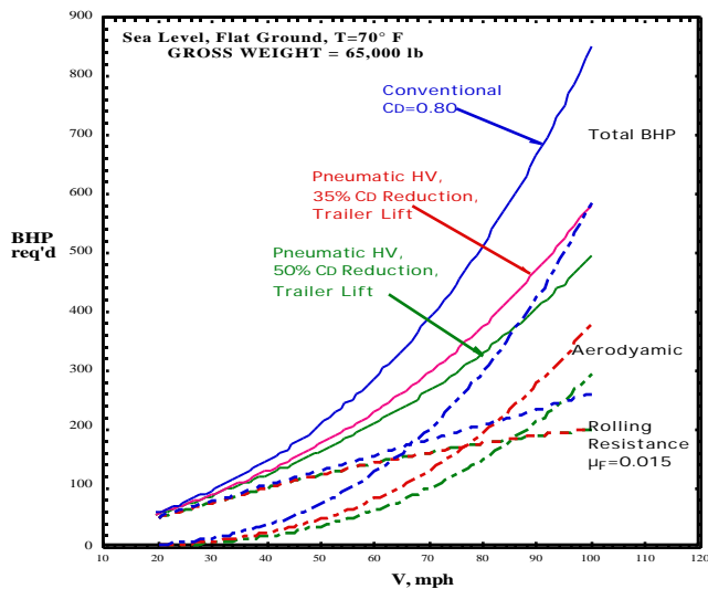
Figure 22 – Comparative Blowing-Produced Reductions in Power Required to Overcome Drag and Rolling Resistance blown vehicles
