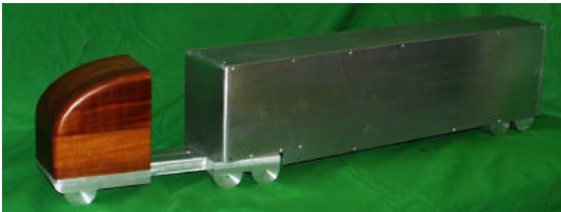
(a) Full-Height Tractor and Yawed Trailer with Rounded Leading Edge and Square Trailing Edge
