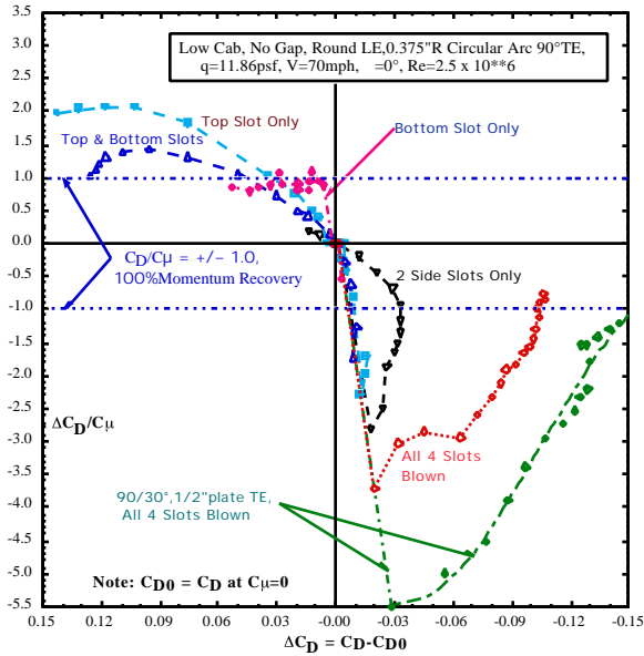
Figure 15 - Blowing Efficiency & Drag Increments due to Blowing Slot Configuration
