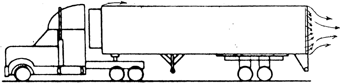
Figure 5 – Schematic of Application of GTRI Pneumatic Aerodynamic Technology to Heavy Vehicle Trailer, Showing 4 Aft Blowing Slots and Upper Leading-Edge Blowing Slot
