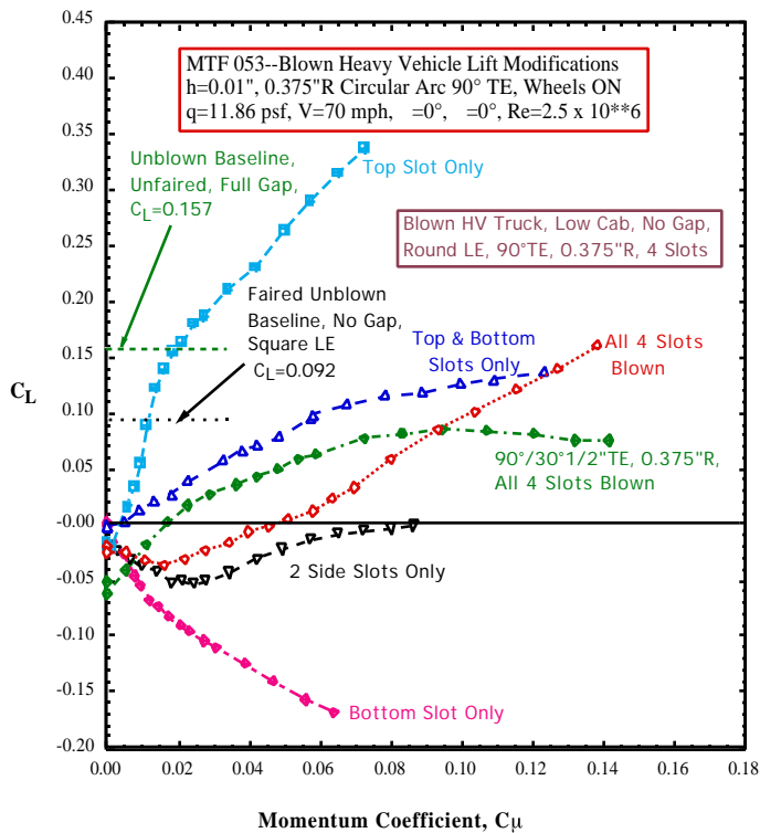
Figure 19 -Lift and Downforce Generation on Blown Trailer with 0.375"R Turning Surface
