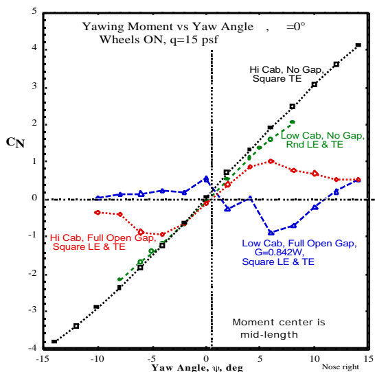
(b.) Yawing Moment about Mid-Length
