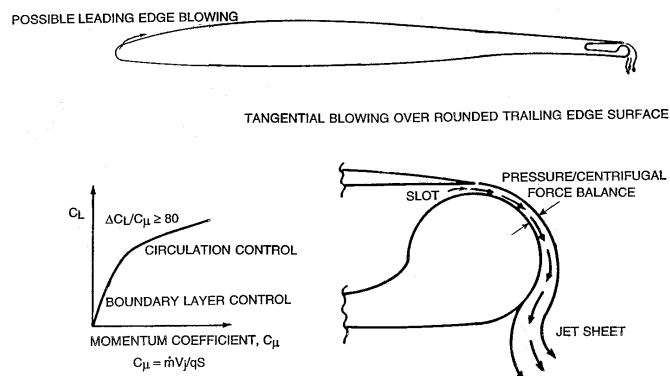
Figure 2 – Basics of Circulation Control Aerodynamics on a Simple 2-D Airfoil
