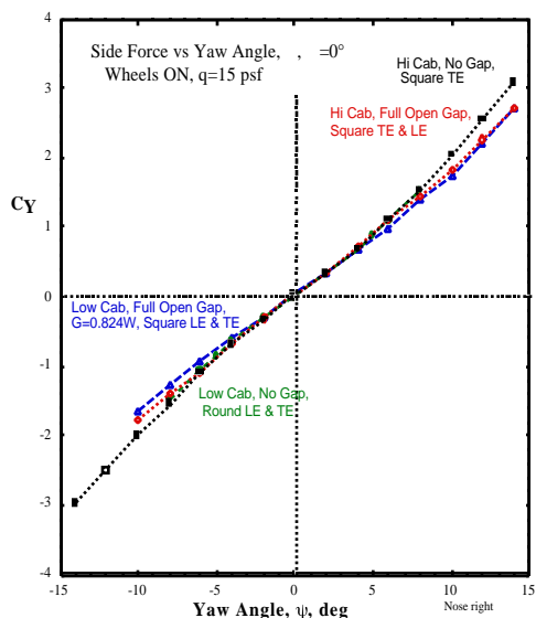
(a.) Side Force
