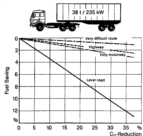
Figure 1 – Effect of Drag Coefficient Reduction on Fuel Consumption (from Ref. 1)
