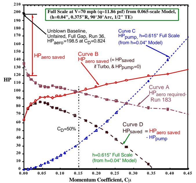
Figure 23 – Horsepower Required to Overcome Drag at 70mph, plus Required Compressor Power and Horsepower Saved
