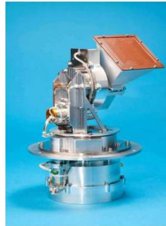
Fig. 7. Antenna pointing mechanism with horn antenna, courtesy of SSTL.
