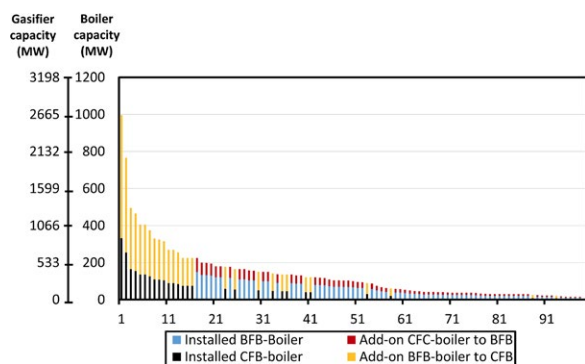
Figure 17. Existing installed capacity of fluidized bed boilers in the Swedish energy system and the corresponding additional boiler sizes needed to realize their conversion to dual fluidized bed gasifiers, Data provided by Christer Gustavsson.
