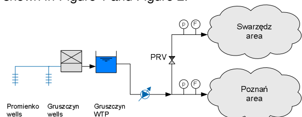
Figure 1: Schematic drawing of the water supply system of Gruszczyn
