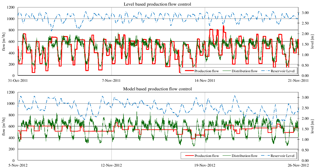
Figure 5: Difference between level based (upper graph) and model based (lower graph) production flow control
