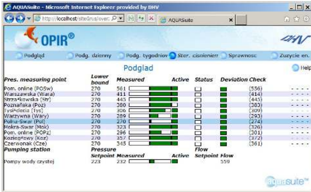
Figure 3: Interface of the dynamic pressure control module (DPCM), showing all measured pressures and their lower bound values, and highlighting which measuring point is the master in the control loop
