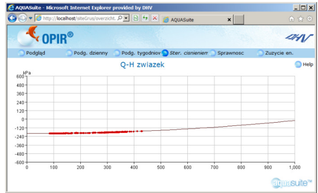
Figure 4: Least squares fit of measured pressure drop between pumping station and pressure measuring point as a relation of the flow to the area
