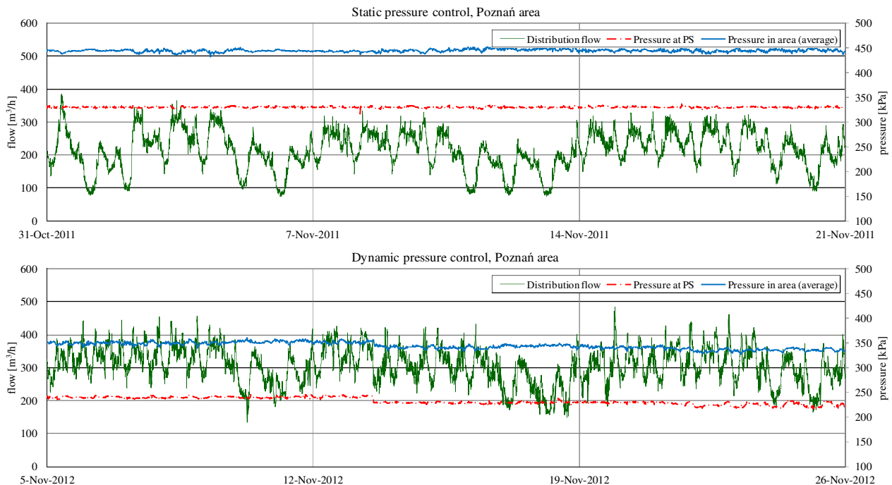
Figure 7: Difference between static (upper graph) and dynamic (lower graph) pressure control, Poznań area
