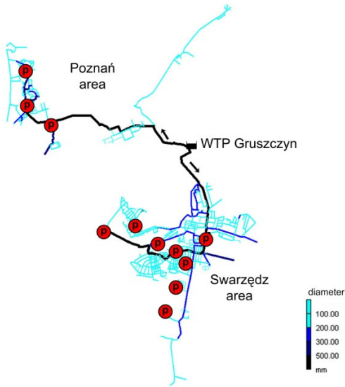
Figure 2: Distribution system of Gruszczyń, including nine new and two existing pressure measuring points
