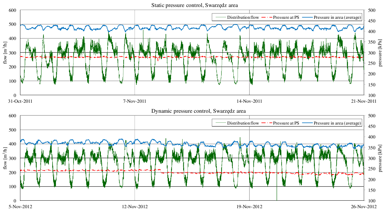
Figure 8: Difference between static (upper graph) and dynamic (lower graph) pressure control, Swarzędz area
