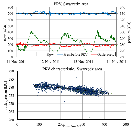
Figure 6: Outlet pressure in the water main to Swarzędz area with conventional pressure control including PRV
