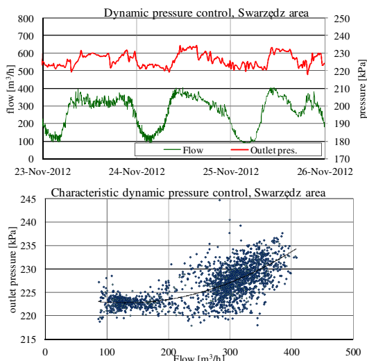
Figure 9: Outlet pressure in the water main to Swarzędz area with dynamic pressure control
