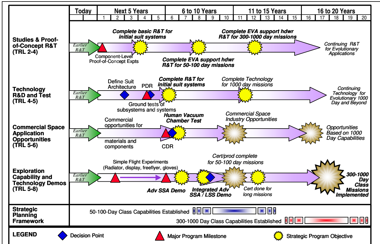
Figure 5.1-1. A general EVA roadmap for HTCI to support similar advanced EVA programs of the type envisioned for this study.
