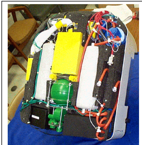
Figure C.1-15. “Foam” advanced PLSS concept.
