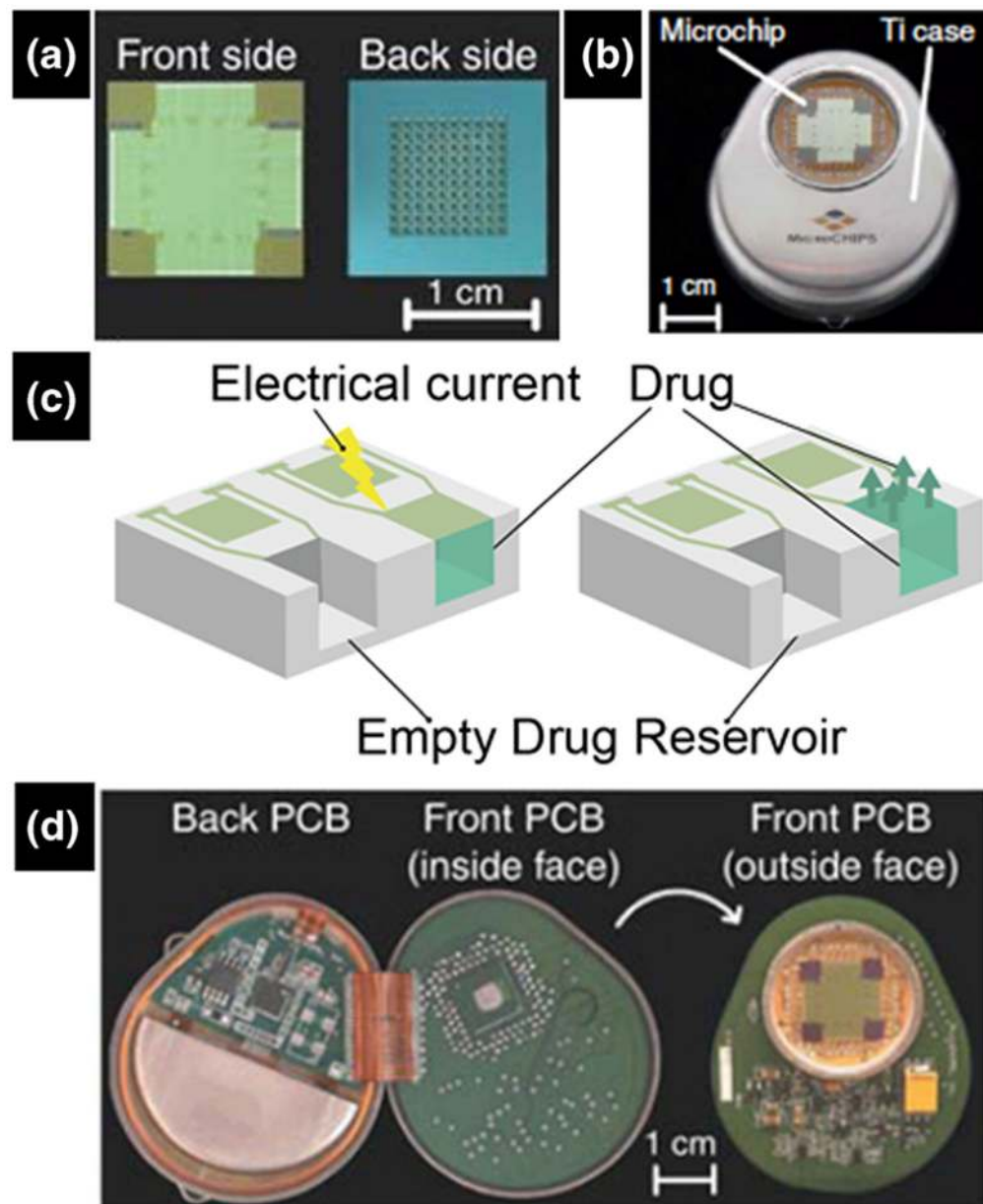
Fig. 6. 30-ml Micro-CHIP device used for leuprolide release in dogs. a Silicon wafer with 100 30 \mu l drug reservoirs capped by gold membranes. b Assembled 30-ml Micro CHIP device. c Micro-CHIP drug release schematic: an electrical potential to the gold membrane permits selective opening of specific reservoir for drug release. d Internal circuitry of the implant. (Image 6A, 6B, 6D adapted from (Prescott et al. 2006))
