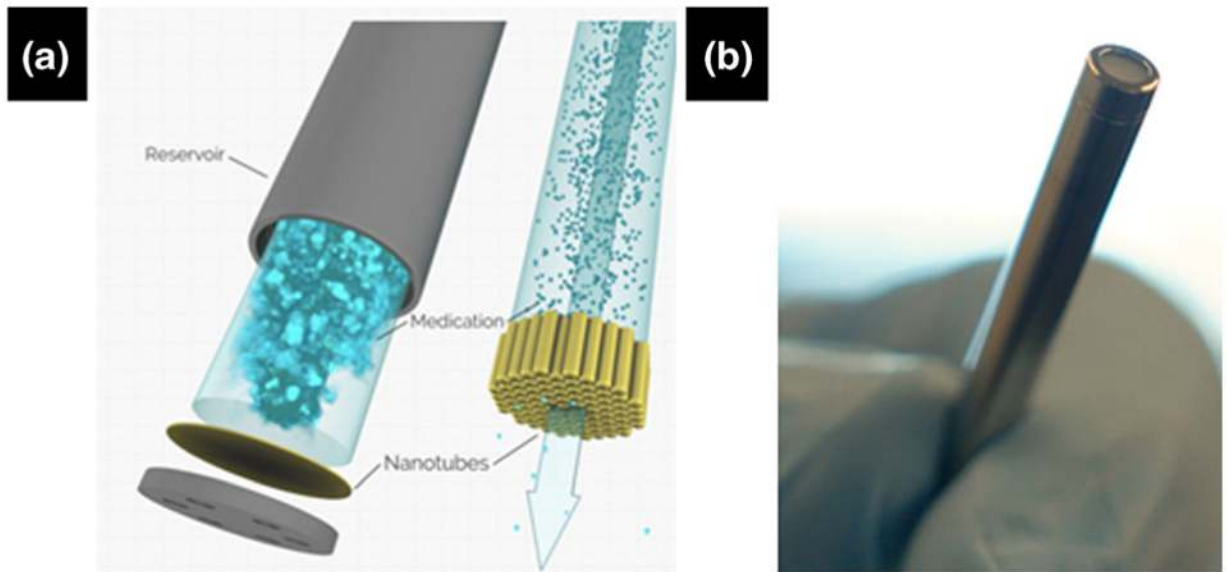
Fig. 8. NEMS translational research devices. a Schematic of nanoportal membrane from Nano Precision Medical showing how the nanotubes are the rate-limiting step for drug release from the reservoir (Image used with permission from Nano Precision Medical). b Drug-versatile Delpor Inc. implant with two membranes with NANOPOR™ technology fixed at each end (Image used with permission from Delpor Inc.)
