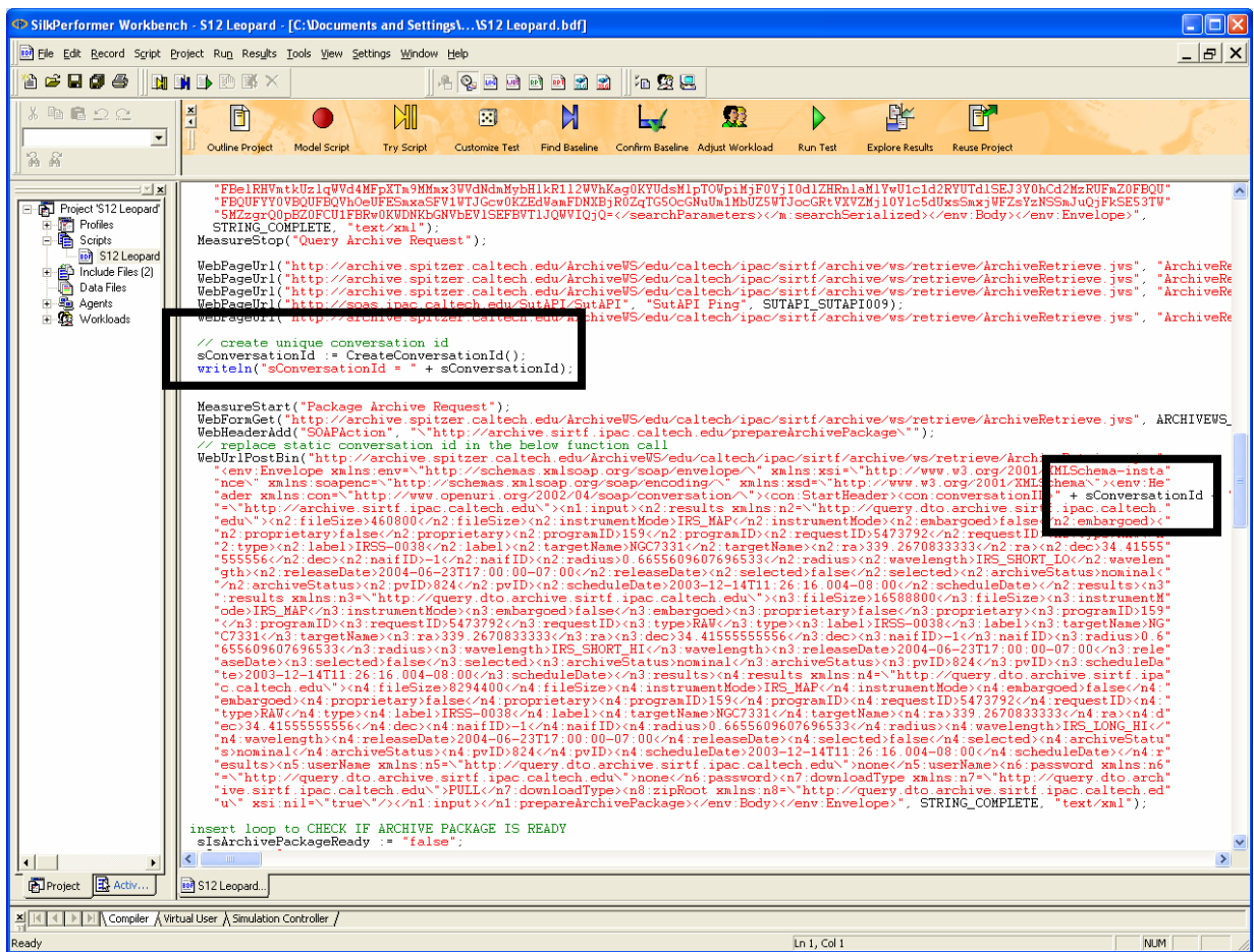
Fig. 5 Load test script showing the manual replacement of the static conversation ID with a variable
