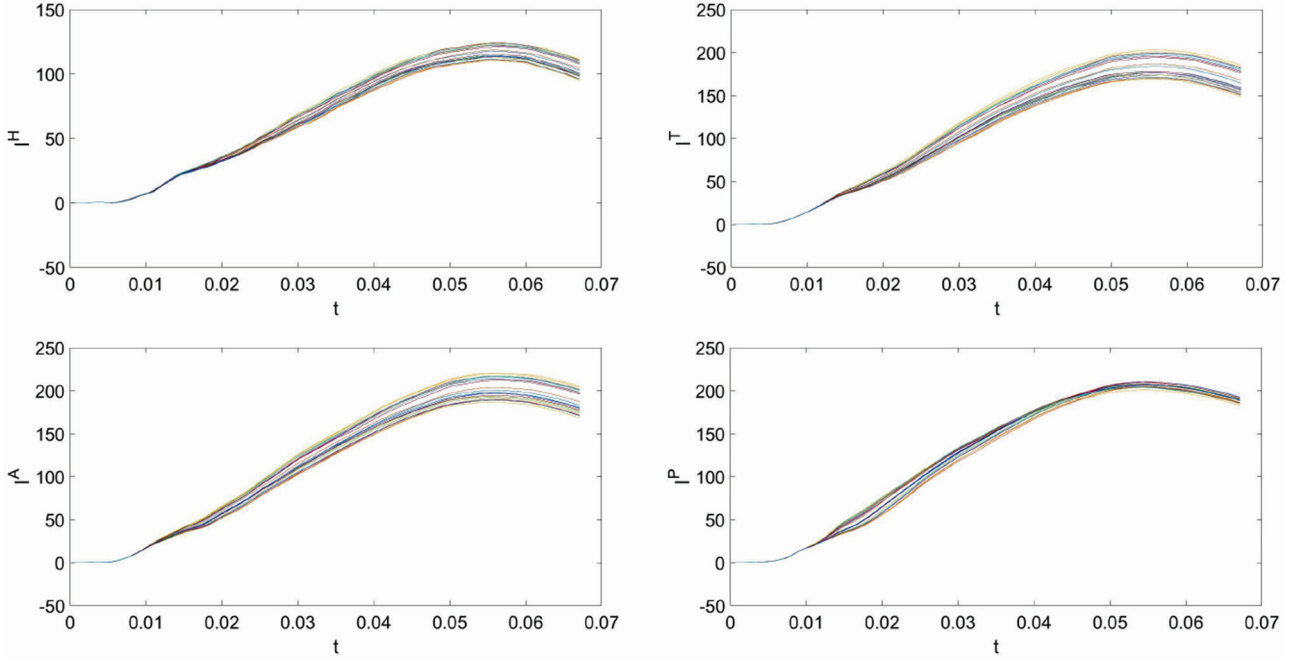
Fig. 9. Temporal evolution of the intrusion I at four different locations of the B-Pillar: I^H , I^T , I^A , & I^P .
