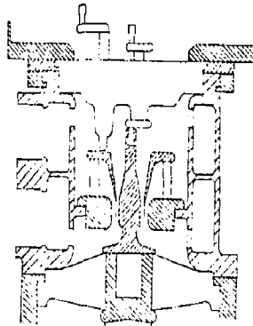
FIGURE 4 SPARK GAP
