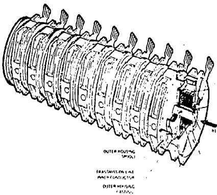
FIGURE 5 ACCELERATOR TEN CELL UNIT
