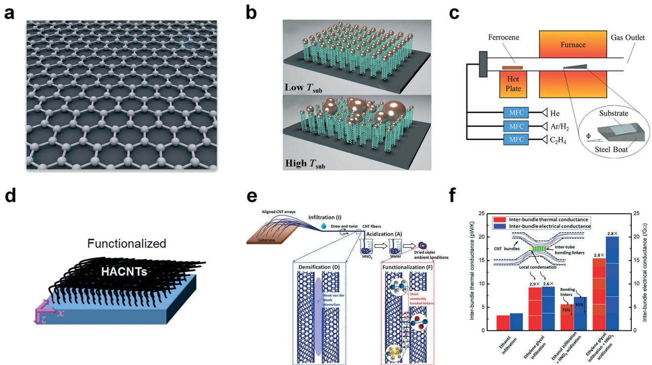
Fig. 2 The thermal properties enhancement of carbon nanomaterials-based TIMs. Scheme of a. graphene, b. producing uniform height for CNT arrays (reprinted with permission from 13 Copyright Elsevier Carbon), c. controlling the tube diameter, array length and reduce the amount of amorphous carbon for CNT array synthesis during chemical vapor deposition process, d. horizontally aligned CNT arrays (reprinted with permission from 14 Copyright John Wiley and Sons Physics Status Solidi A-Applications and Materials Science ), e. functionalization and densification of inter-bundle interface (reprinted with permission from 16 Copyright Elsevier Carbon). f. boosted inter-bundle interfacial thermal and electrical conductance for functionalized and condensed CNT fibers (reprinted with permission from 16 Copyright Elsevier Carbon).
