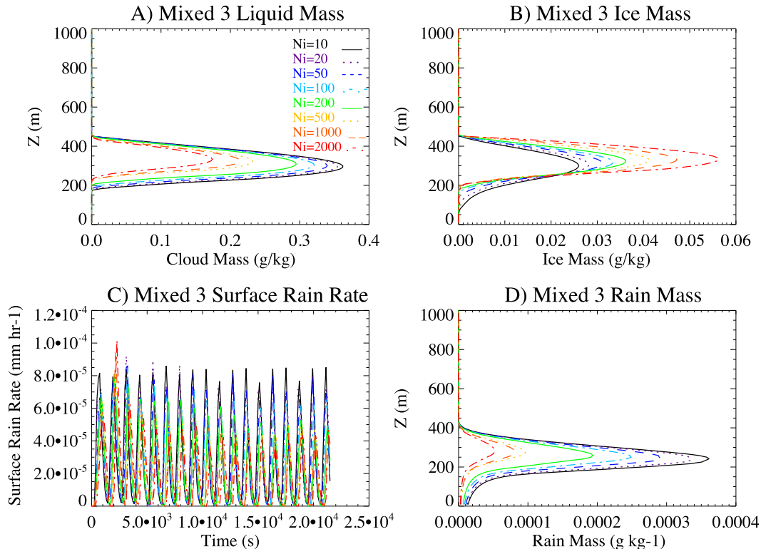
FIG. 13. Mixed 3 case comparisons with MG2 of temporally averaged (a) cloud liquid mass, (b) cloud ice mass, (c) surface rain rate (not temporally averaged), and (d) rain mass with different number concentrations for ice crystals (colored lines) from 10 to 2000 L -1 . Fixed drop number of N_c = 100 \text{ cm}^{-2} .
