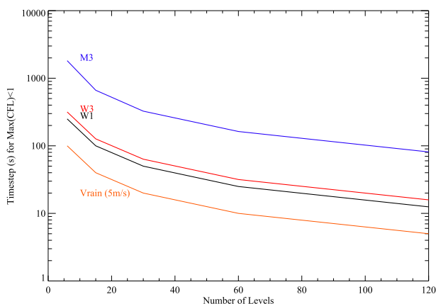
FIG. 1. Maximum time step for maintaining \text{CFL} < 1 for cases Warm 1 (W1), Warm 3 (W3), and Mixed 3 (M3) and for a fall speed for rain ( V_{\text{rain}} ) of 5 \text{ m s}^{-1} .
