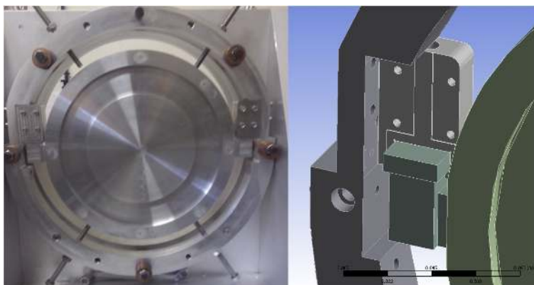
Figure 9. Prototype of the Compensation Plate suspension and detail of the lateral clamps.
