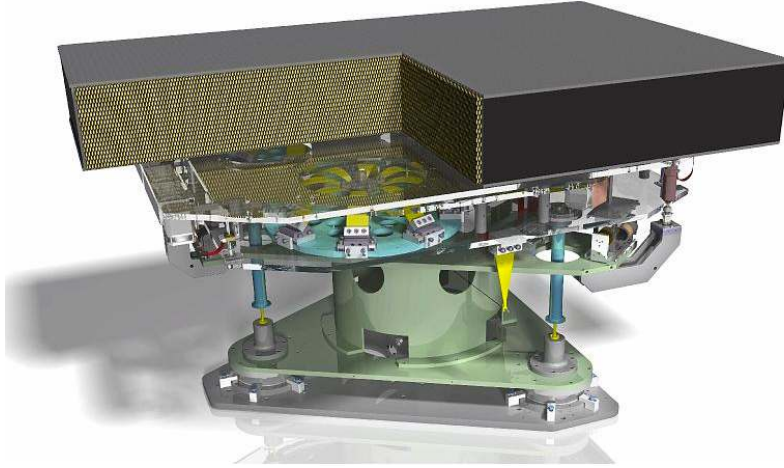
Figure 16. Impression of the External Injection Bench supported by the EIB-SAS. The EIB is a standard 2400×1500-mm optical bench with a mass of 840 kg. The inverted pendulum legs allow the intermediate platform (spring-box) to move horizontally. The spring-box hosts the three GAS springs, which allow the optical bench to move along vertical, pitch and roll degrees of freedom.
