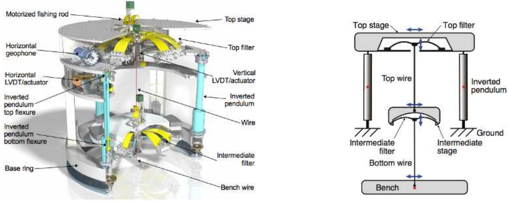
Figure 26. Left panel: MultiSAS overview. Right panel: MultiSAS conceptual design; two vertical (GAS springs) and three horizontal (IP and two simple pendulums) isolation stages are provided.
