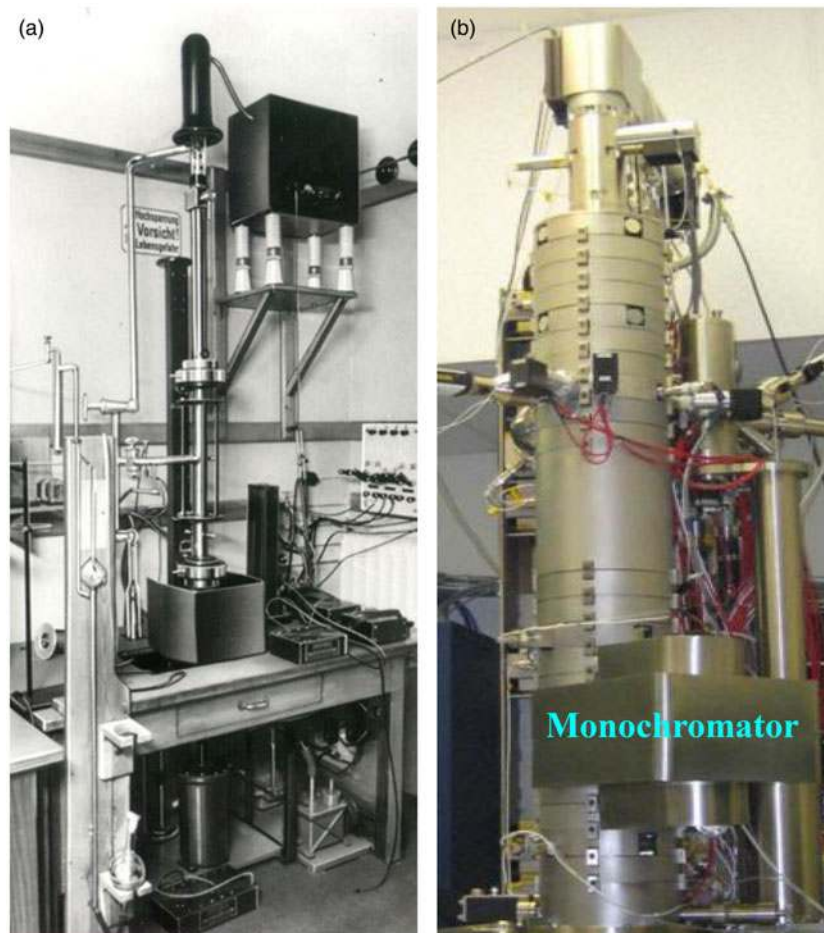
Fig. 2. (a) Manfred von Ardenne developed the first scanning transmission electron microscope (1938), with an electron-beam diameter on target of \sim 10 nm. His first image was a zinc oxide crystal at 8,000\times magnification. Adapted from Science/AAAS Custom Publishing Office ( http://poster.sciencemag.org/sem/# ). (b) The Nion aberration-corrected and monochromated UltraSTEM 100 at Arizona State University: sub-Ångstrom resolution at 60/100 kV, about 1 Ångstrom resolution at 30/40 kV, and 10 meV energy resolution in ultrafast EELS.
