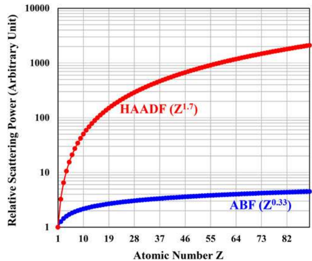
Fig. 13. Plots of the dependence of HAADF ( \sim Z^{1.7} ) and ABF ( \sim Z^{1/3} ) signal strength on the atomic number Z .
