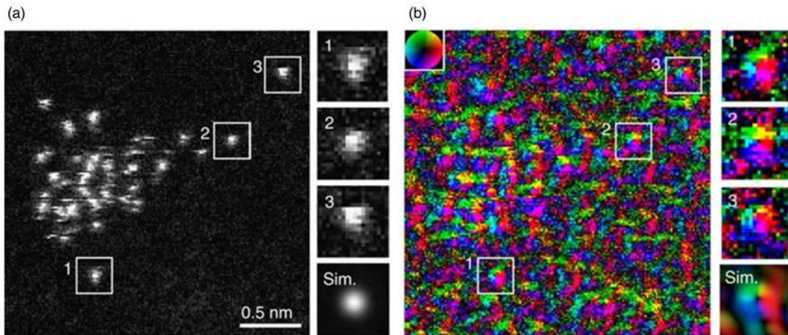
Fig. 14. Simultaneous atomic-resolution ADF STEM image (a) and electric field vector map (b) of Au single atoms. The dwell time is 300 \mu\text{s} per pixel. The inset color wheel indicates how color and shade denote the electric field orientation and strength. Magnified images from three isolated Au atom positions are indicated. Simulated image of a single Au atom supported on a 10 nm-thick amorphous carbon substrate is also shown. Reproduced from Shibata et al. (2017).
