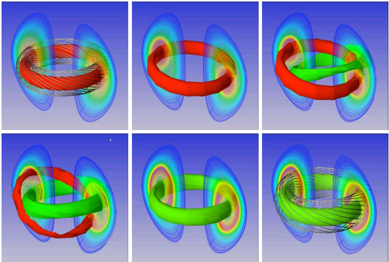
Figure 7. Simulation of the nonlinear evolution of an internal magnetic reconnection event in the National Spherical Torus Experiment.
