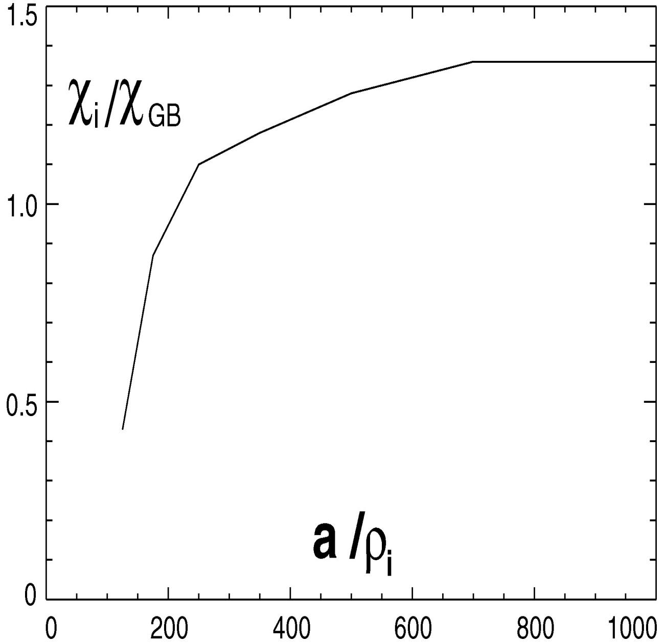
Figure 11. Full torus particle-in-cell gyrokinetic simulations (GTC) of turbulent transport scaling.
