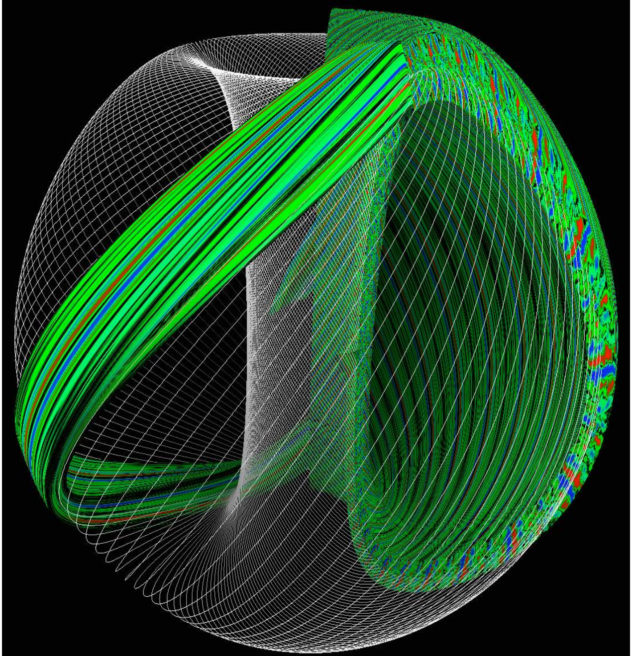
Figure 9. Flux-tube simulation results of turbulence localized to an annular region of a 3D toroidal plasma.
