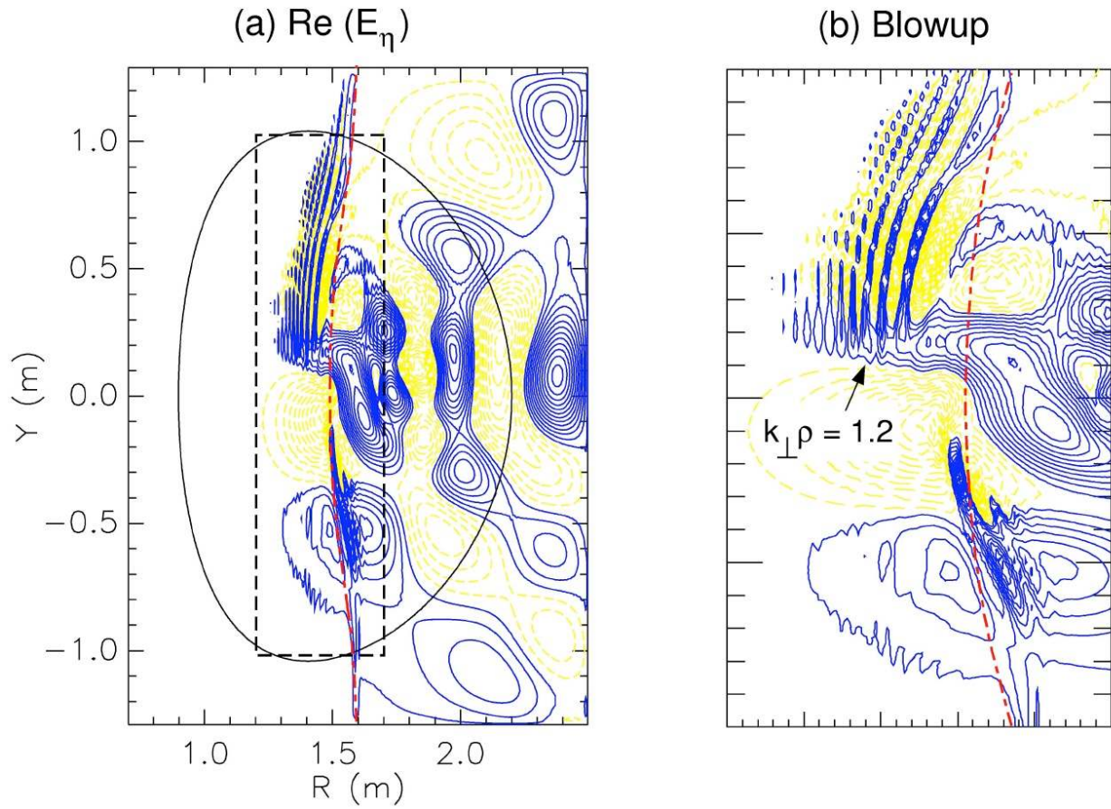
Figure 14. Two-dimensional field solutions for conversion of fast ion cyclotron waves to ion Bernstein waves in the heating of the DIII-D tokamak plasma.
