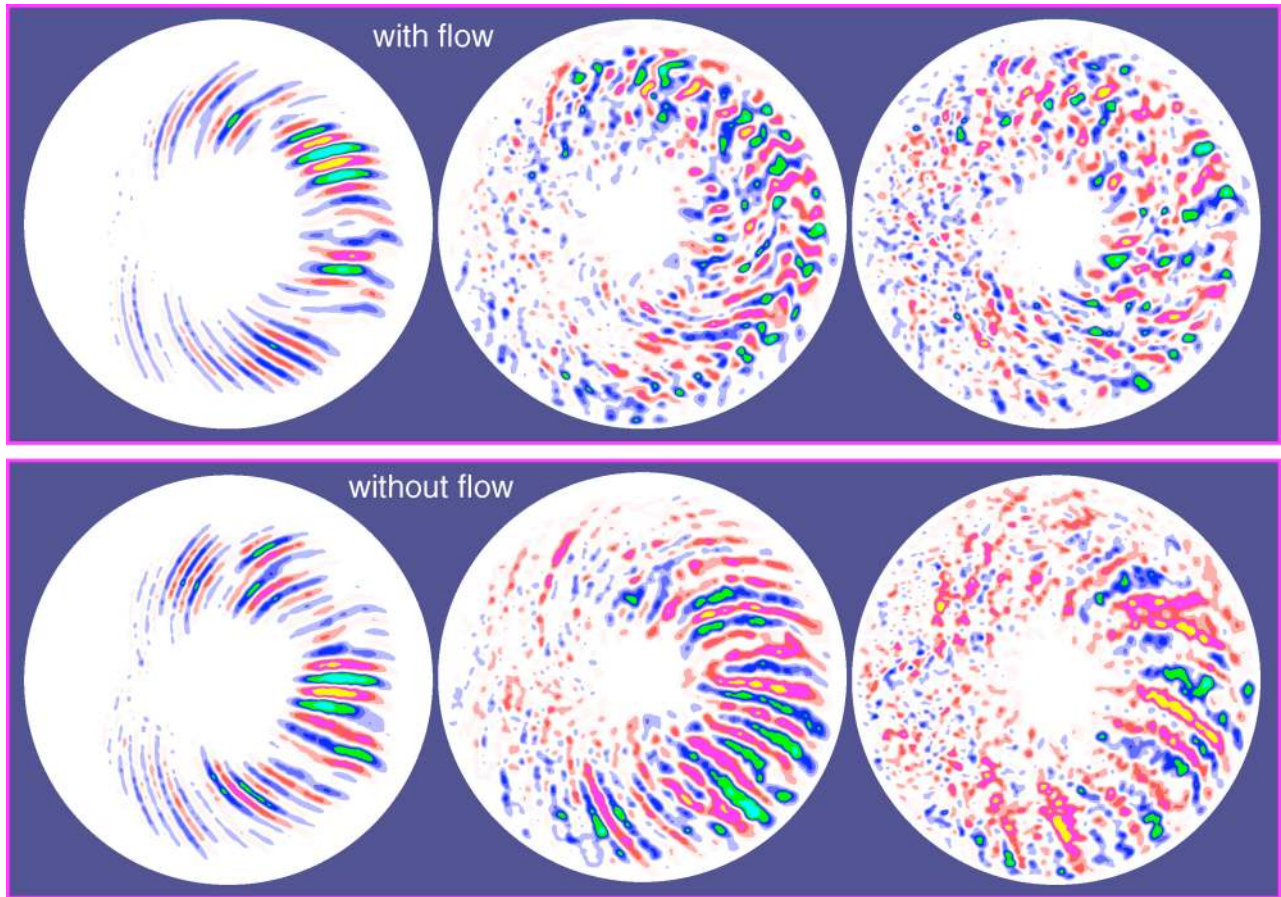
Figure 10. Turbulence reduction via sheared plasma flow compared to case with flow suppressed.
