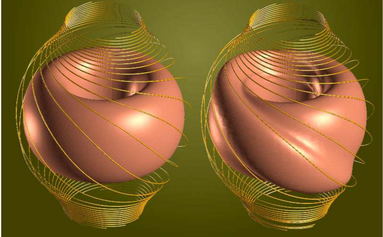
Figure 8. Simulation of the nonlinear evolution of an internal magnetic reconnection event in the START spherical torus experiment.
