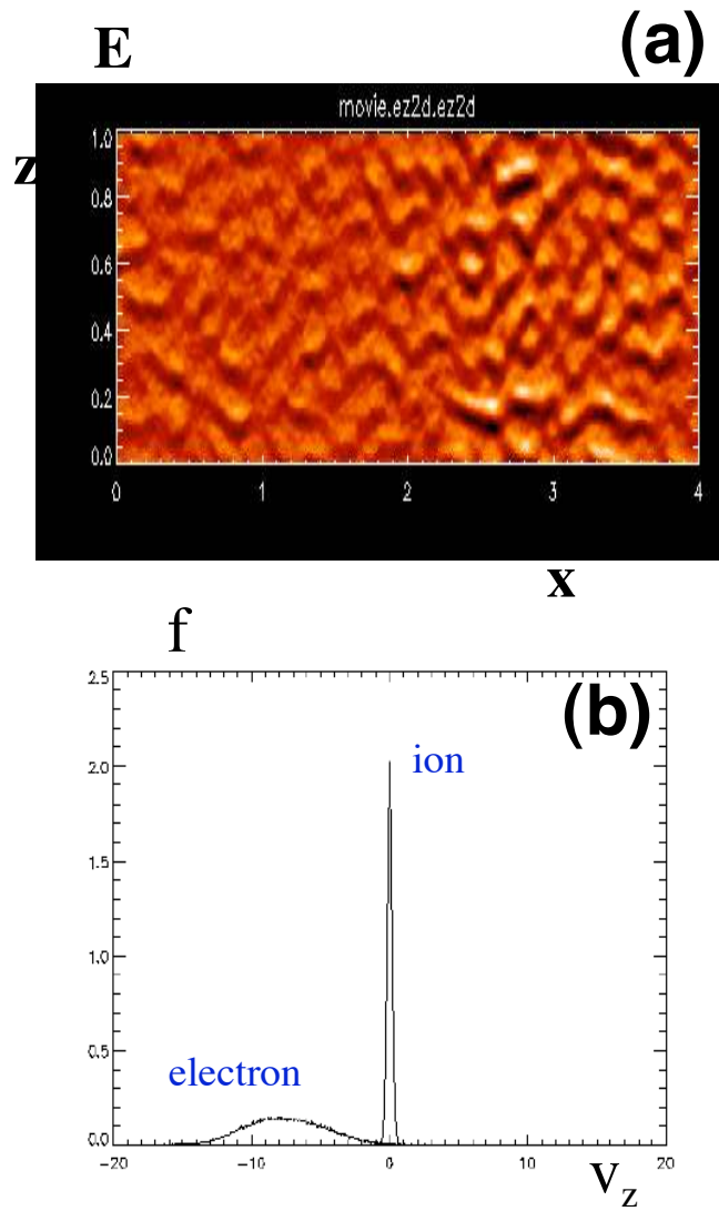
Figure 19. 3D particle-in-cell code simulations of dynamics in the magnetic reconnection current layer leading to the generation of localized regions of intense anti-parallel electric field (“electron holes”).
