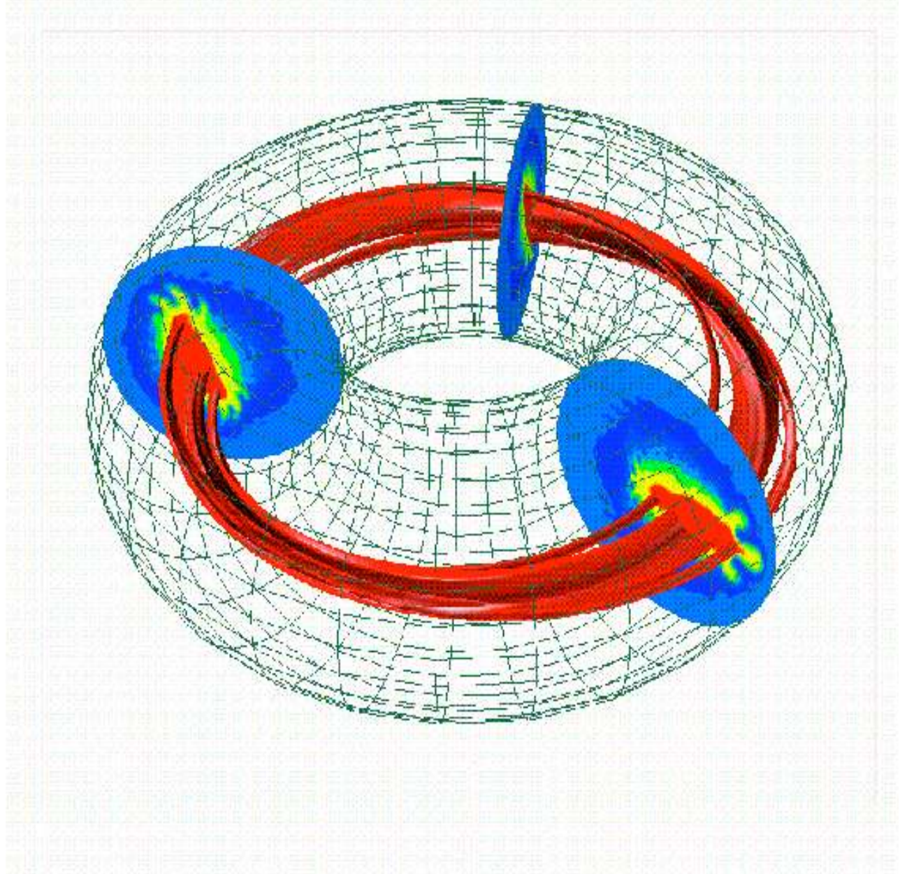
Figure 5. Three-dimensional nonlinear macroscopic simulation of a disruption event in the TFTR tokamak experiment.
