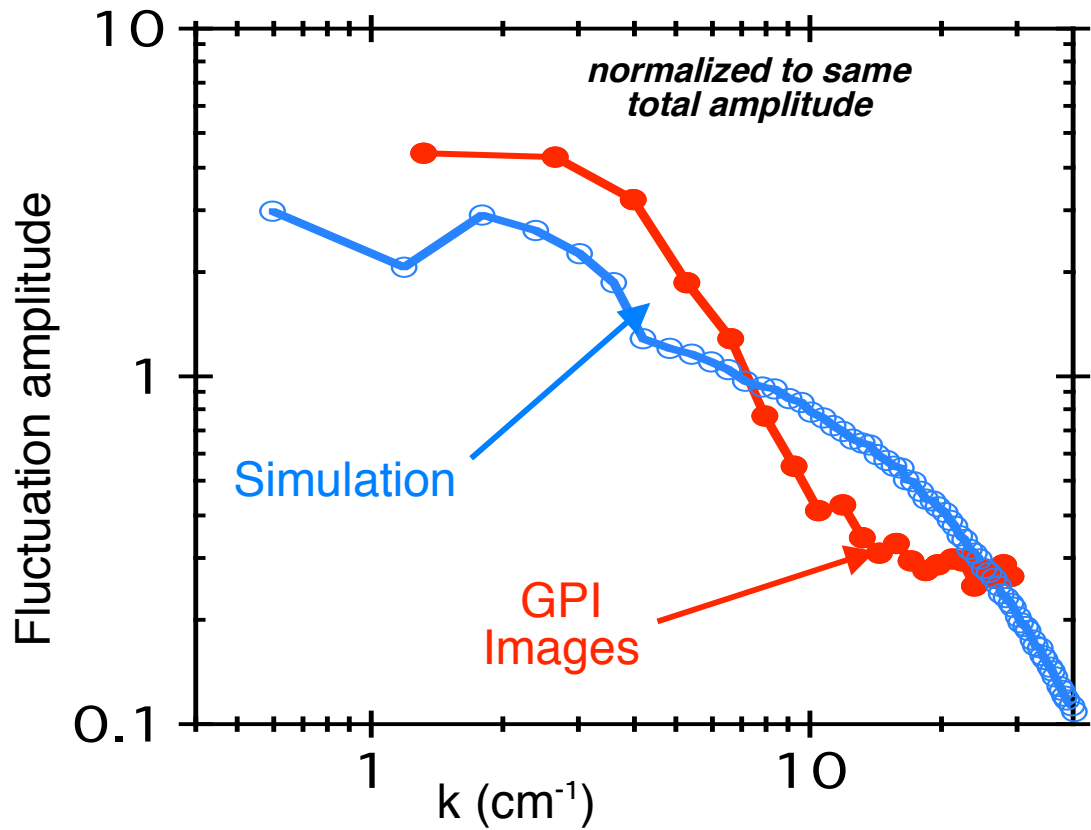
Figure 16. Wave number ( k ) spectrum comparisons between Gas-Puff Imaging (GPI) experimental measurements and 3D electromagnetic fluid code simulations of edge turbulence on the Alcator C-Mod tokamak.
