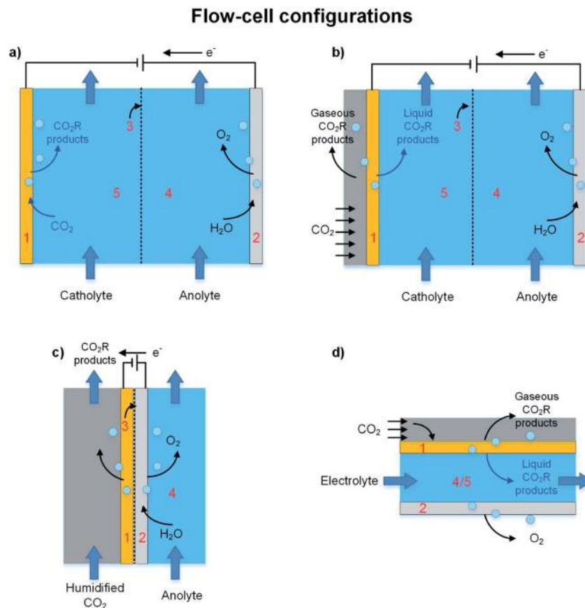
Fig. 5 Schematic of CO 2 electrolyzer in flow-cell configurations (a and b) liquid-fed electrolyzer, (c) vapor-fed electrolyzer and (d) microfluidic reactor. The main cell components are labelled as (1) cathode, (2) anode, (3) separator or ion-exchange membrane which could be a cation exchange membrane, anion exchange membrane, or a bipolar membrane, (4) anolyte, and (5) catholyte.
