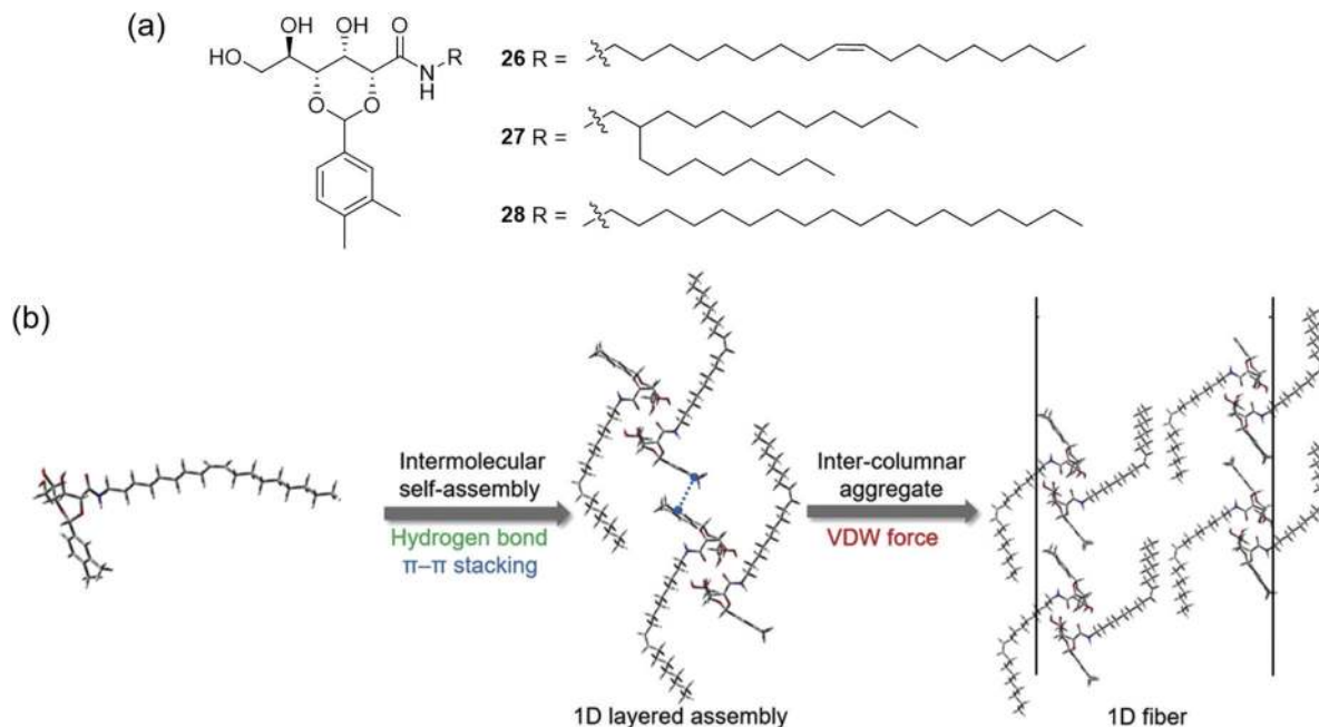
Fig. 22 (a) The structure of gelators 26–28 ; (b) Gelation of hydrophobic solvents occurs via the formation of intermolecular hydrogen bonds, \pi\text{-}\pi stacking and van der Waals interactions between lipophilic chains. 149 Adapted from ref. 149 with permission from Elsevier, copyright 2020.
