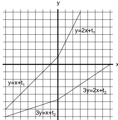
Fig. 2. Broken lines corresponding to S = \{(1, 1), (3, 1)\} and c = 2 .
