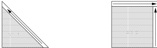
Figure 1: Scheduling wavefront computations by “diagonal” and “square” shells.
